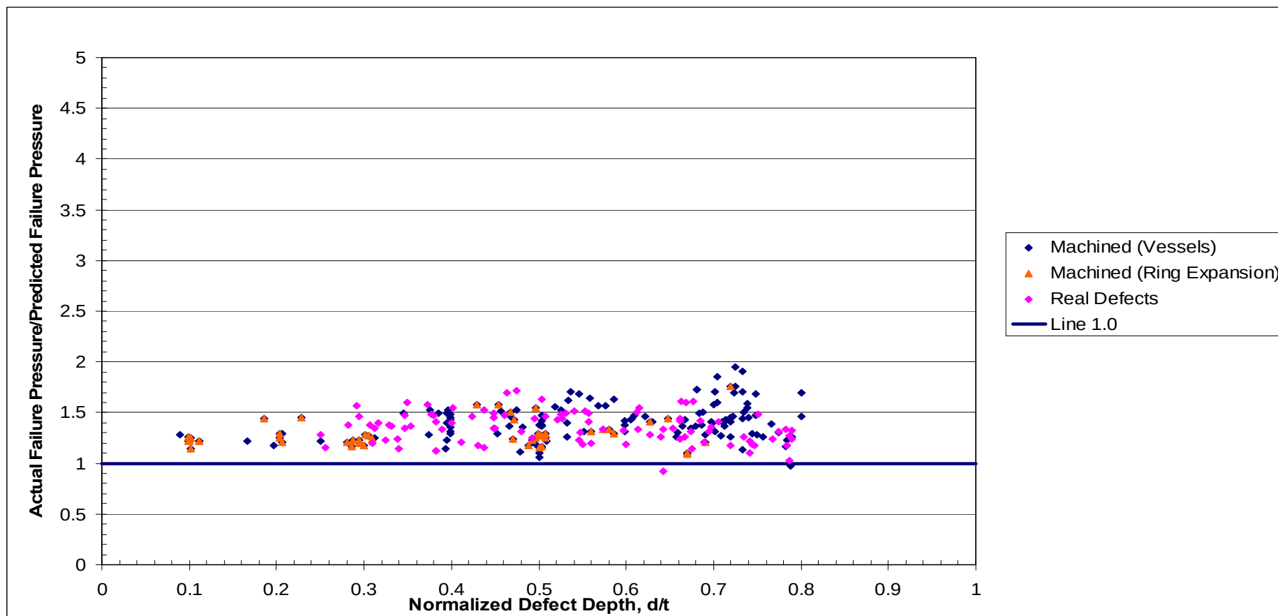
Figure 58 Case 6 Assessments - Comparison of Actual and Predicted Failure Pressure Using the RSTRENG Method (Flow Stress Modified to Equal the Mean of the Specified Minimum Tensile and Ultimate Tensile Strength) – Split Between Machined and Real Corrosion Defects
