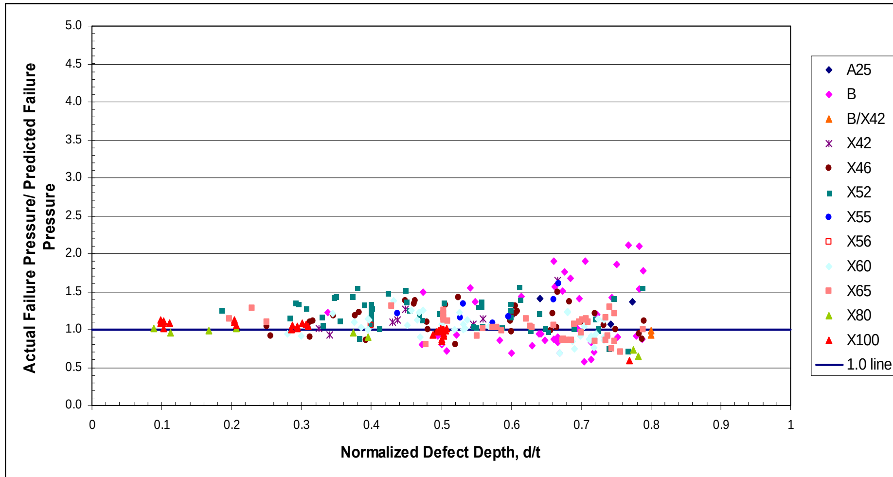
Figure 38 Case 3 Assessments - Comparison of Actual and Predicted Failure Pressures for the Integrated Test Database Using the ASME B31G Method (Flow Stress Modified to Equal the Actual Tensile Strength)
