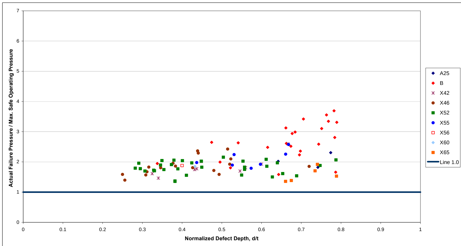
Figure 30 Case 2 Assessments with Factor of Safety 1.25 - Comparison of Actual and Maximum Safe Operating Pressures Using the Modified ASME B31G Method - Real Corrosion Defects
