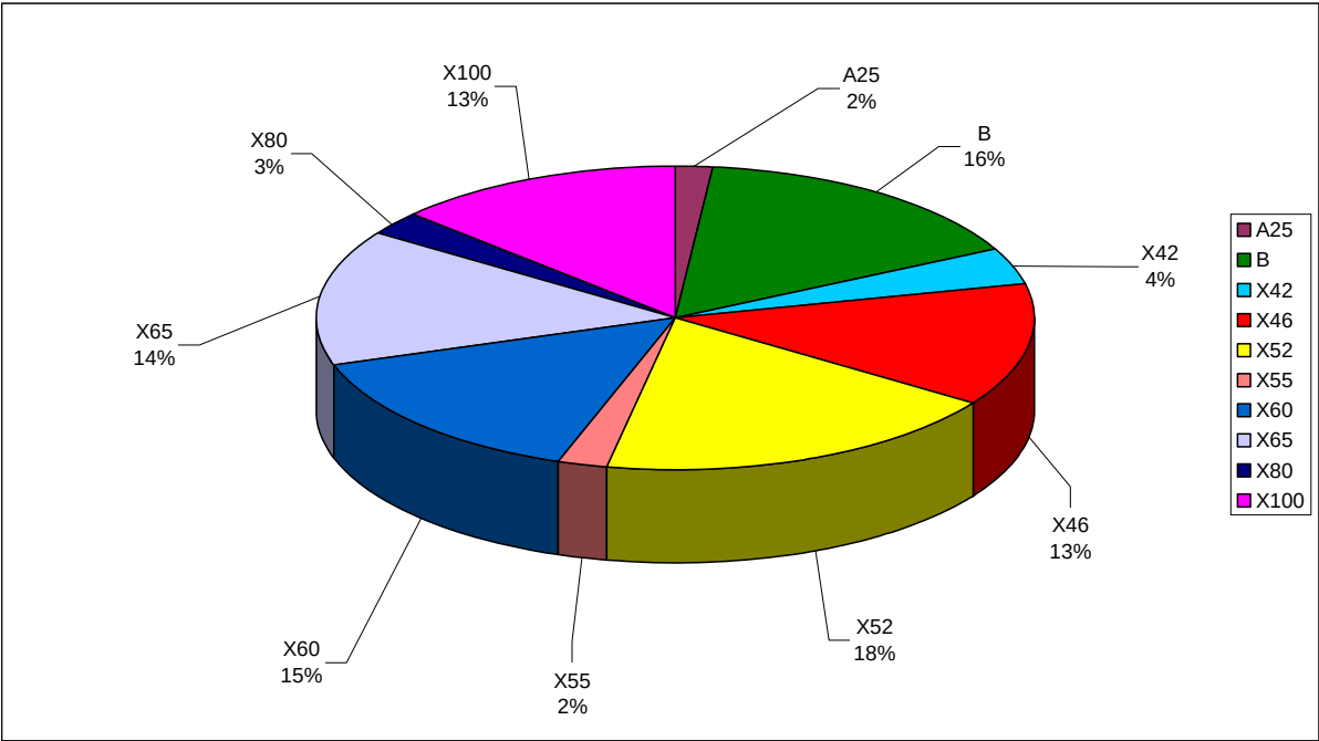
Figure 1 Material Grades Covered in the Integrated Burst Test Database
