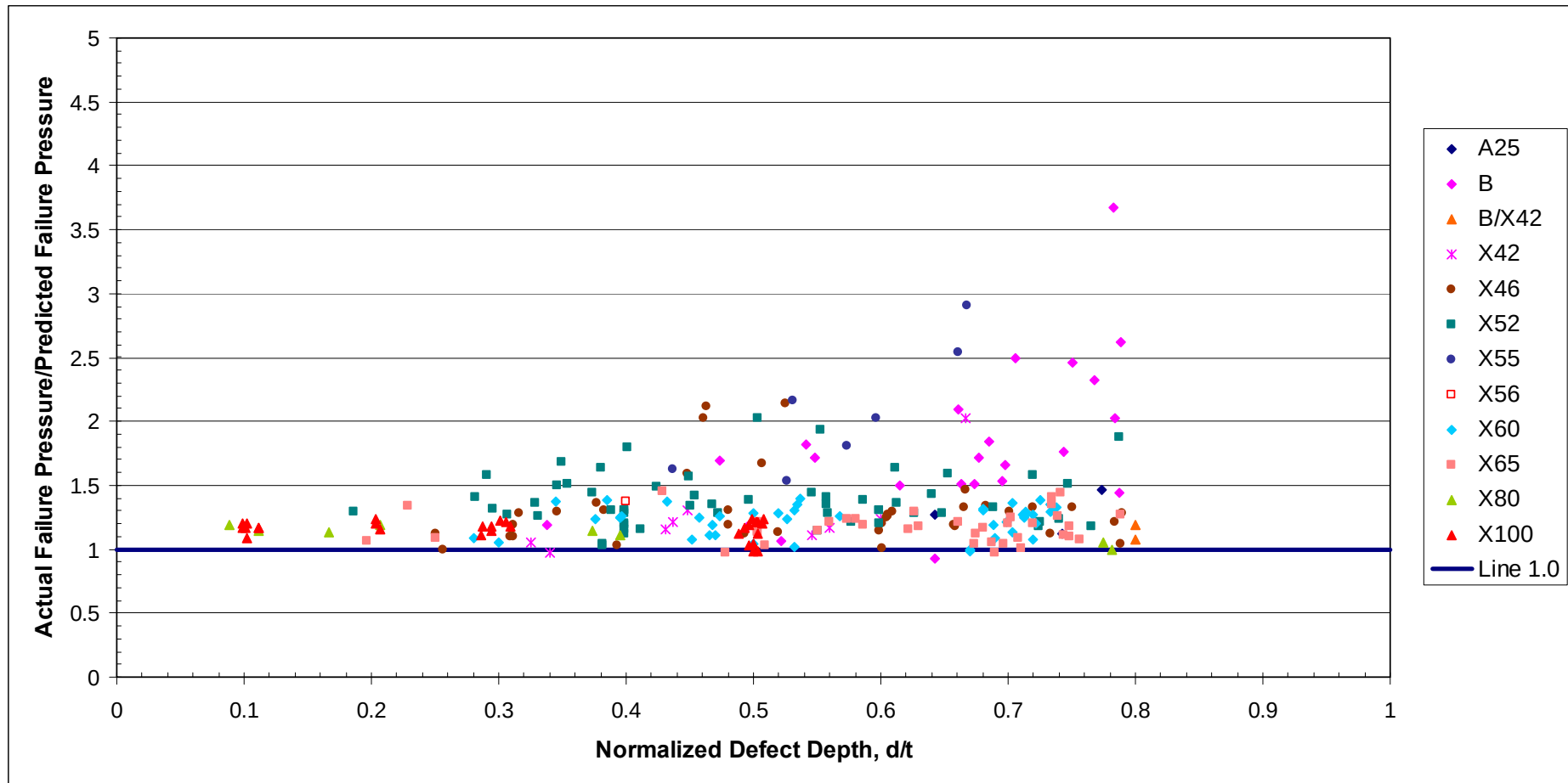
Figure 21 Case 2 Assessments Without a Factor of Safety - Comparison of Actual and Predicted Failure Pressures for the Integrated Database Using the PCORRC Method
