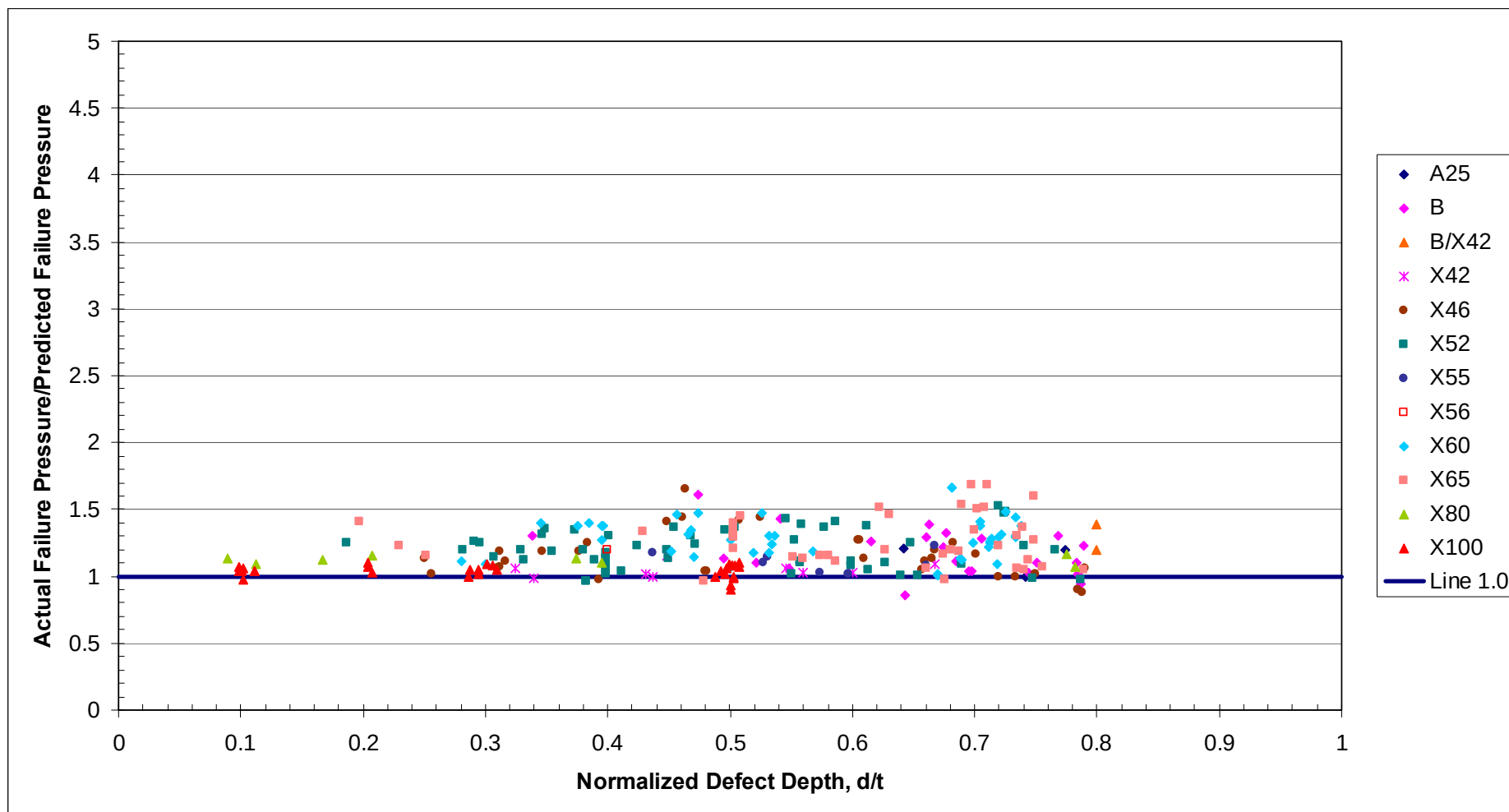
Figure 6 Case 1 Assessments - Comparison of Actual and Predicted Failure Pressure for the Integrated Test Database Using the RSTRENG Method
