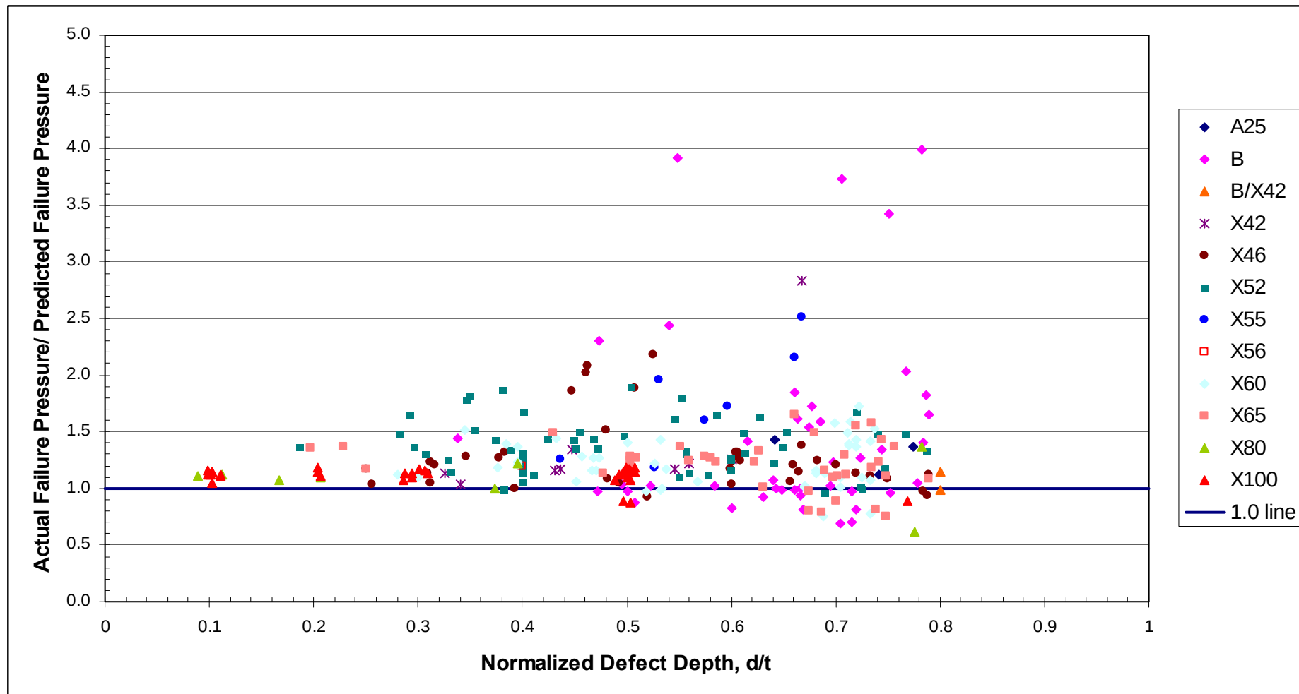
Figure 44 Case 5 Assessments - Comparison of Actual and Predicted Failure Pressures for the Integrated Test Database Using the ASME B31G Method (Flow Stress Modified to Equal the Mean of the Actual Tensile and Ultimate Tensile Strength)
