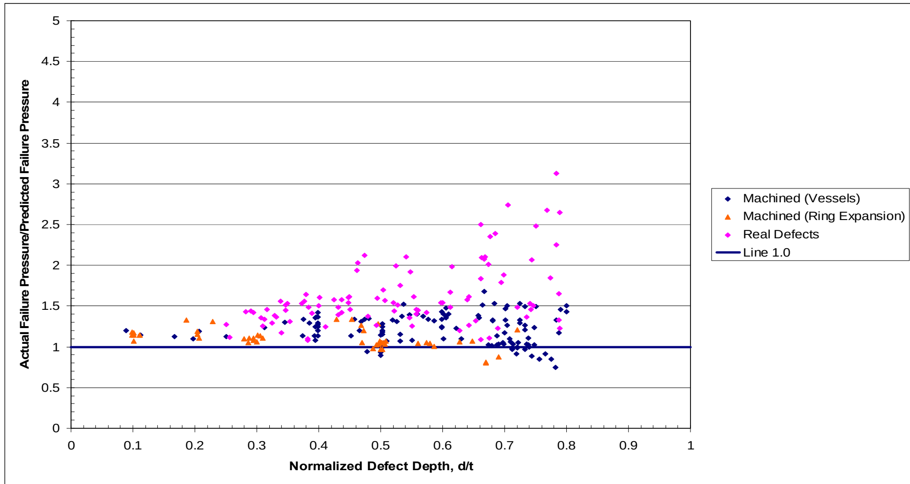
Figure 23 Case 2 Assessments Without a Factor of Safety - Comparison of Actual and Predicted Failure Pressures for the Integrated Database Using the Modified ASME B31G Method including Ring Expansion Tests) – Split Between Machined and Real Corrosion Defects
