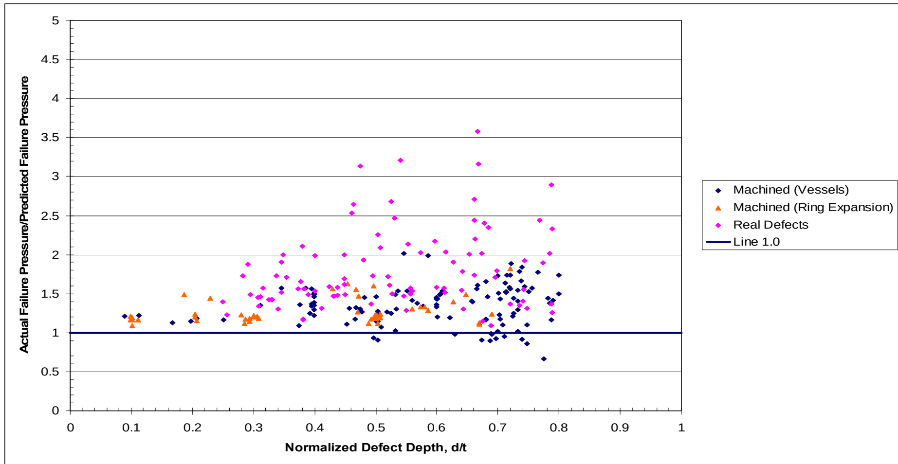
Figure 22 Case 2 Assessments Without a Factor of Safety - Comparison of Actual and Predicted Failure Pressures for the Integrated Database Using the ASME B31G Method- Split Between Machined and Real Corrosion Defects
