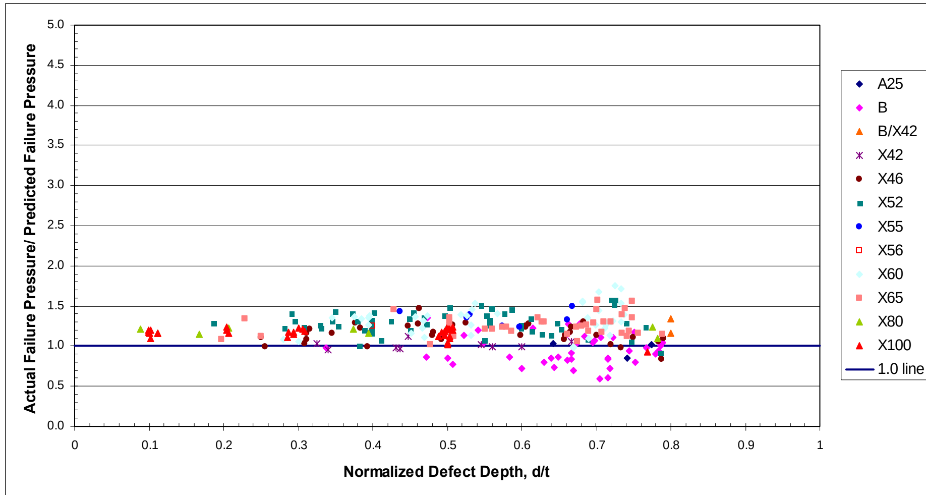
Figure 43 Case 4 Assessments - Comparison of Actual and Predicted Failure Pressures for the Integrated Test Database Using the RSTRENG Method (Flow Stress Modified to Equal the Specified Minimum Tensile Strength)
