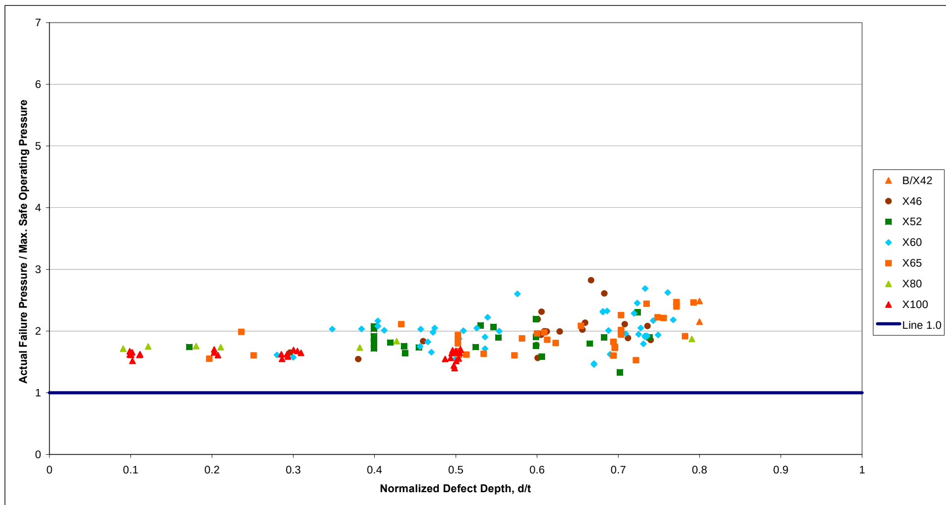
Figure 36 Case 2 Assessments with Factor of Safety 1.39 - Comparison of Actual and Maximum Safe Operating Pressures Using the Modified ASME B31G Method - Machined Defects
