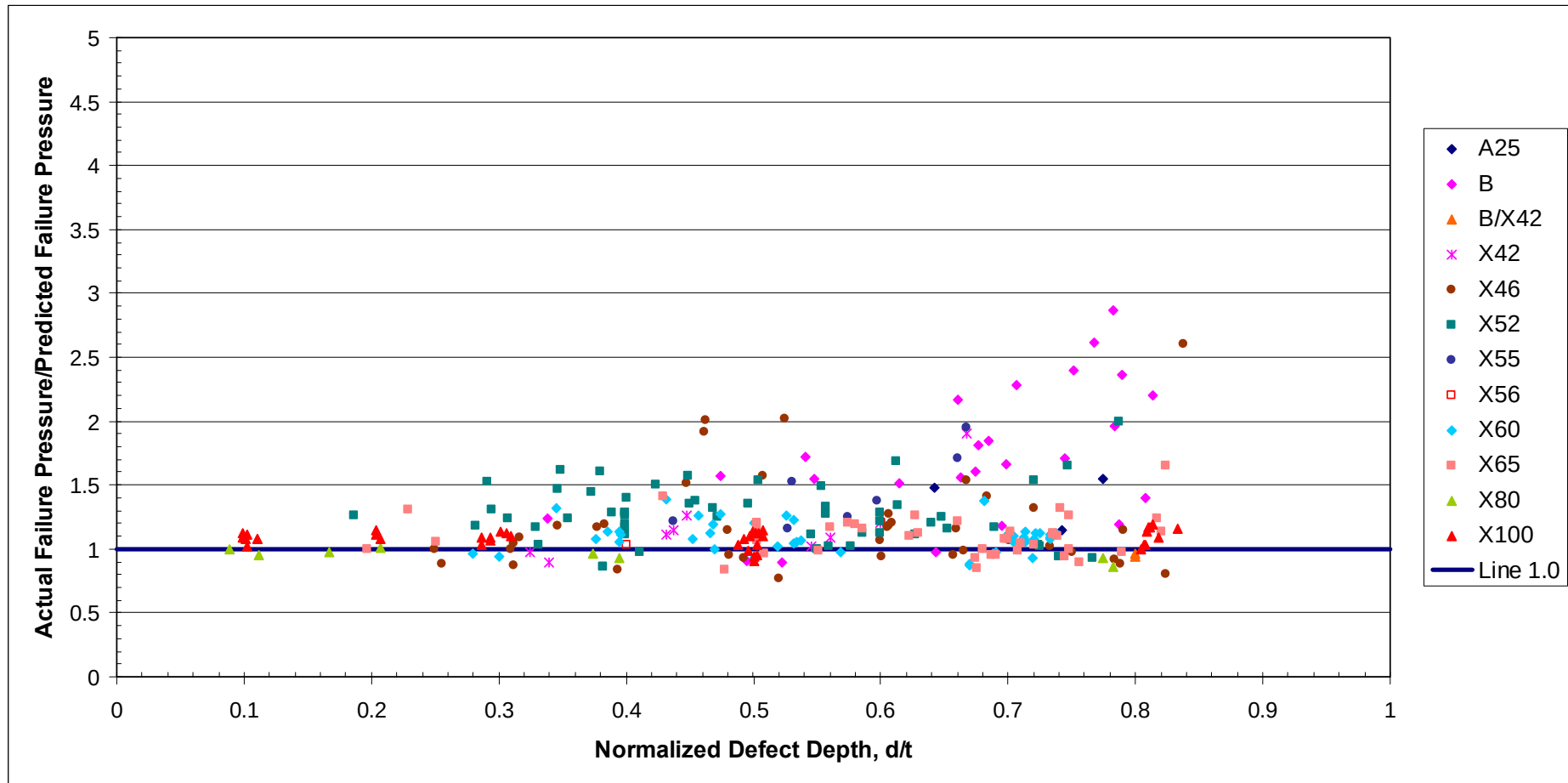
Figure 7 Case 1 Assessments - Comparison of Actual and Predicted Failure Pressure for the Integrated Test Database Using the LPC-1 Method
