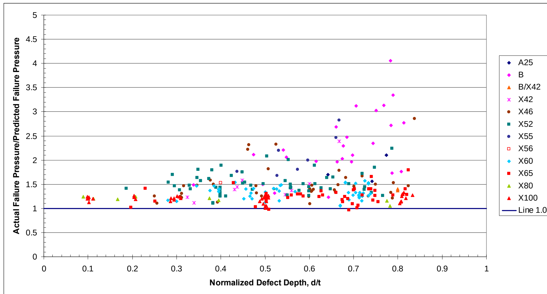
Figure 53 Case 6 Assessments - Comparison of Actual and Predicted Failure Pressures Using the LPC-1 Method (Flow Stress Modified to Equal the Mean of the Specified Minimum Tensile and Ultimate Tensile Strength)
