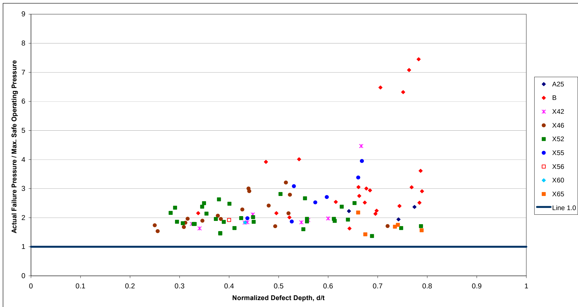
Figure 28 Case 2 Assessments with Factor of Safety 1.25 - Comparison of Actual and Maximum Safe Operating Pressures Using the ASME B3G Method - Real Corrosion Defects
