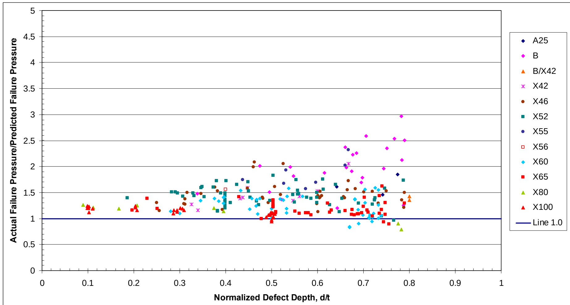
Figure 51 Case 6 Assessments - Comparison of Actual and Predicted Failure Pressures Using the Modified ASME B31G Method (Flow Stress Modified to Equal the Mean of the Specified Minimum Tensile and Ultimate Tensile Strength, including Ring Expansion Tests)
