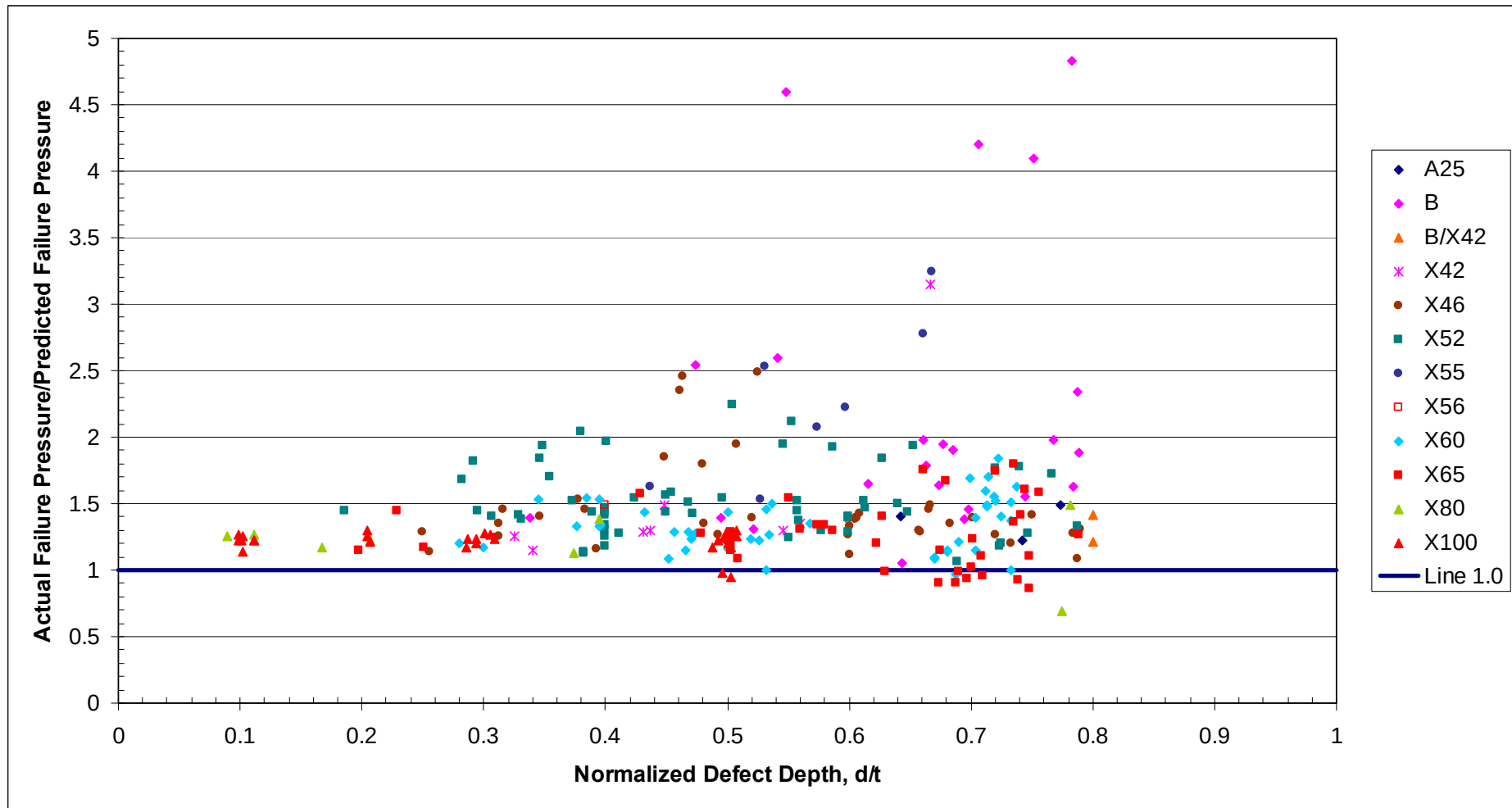
Figure 50 Case 6 Assessments - Comparison of Actual and Predicted Failure Pressures Using the ASME B31G Method (Flow Stress Modified to Equal the Mean of the Specified Minimum Tensile and Ultimate Tensile Strength)
