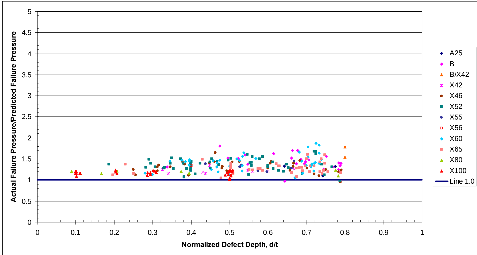
Figure 18 Case 2 Assessments Without a Factor of Safety - Comparison of Actual and Predicted Failure Pressures for the Integrated Database Using the RSTRENG Method
