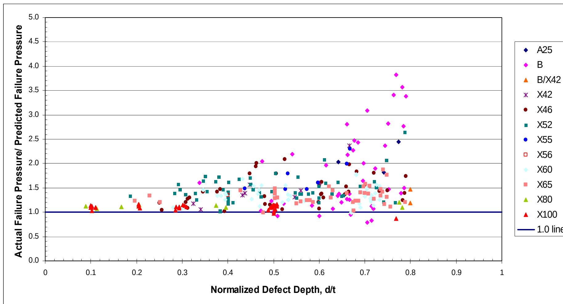
Figure 48 Case 5 Assessments - Comparison of Actual and Predicted Failure Pressure Using the SHELL92 Method (Flow Stress Modified to Equal the Mean of the Actual Tensile and Ultimate Tensile Strength)
