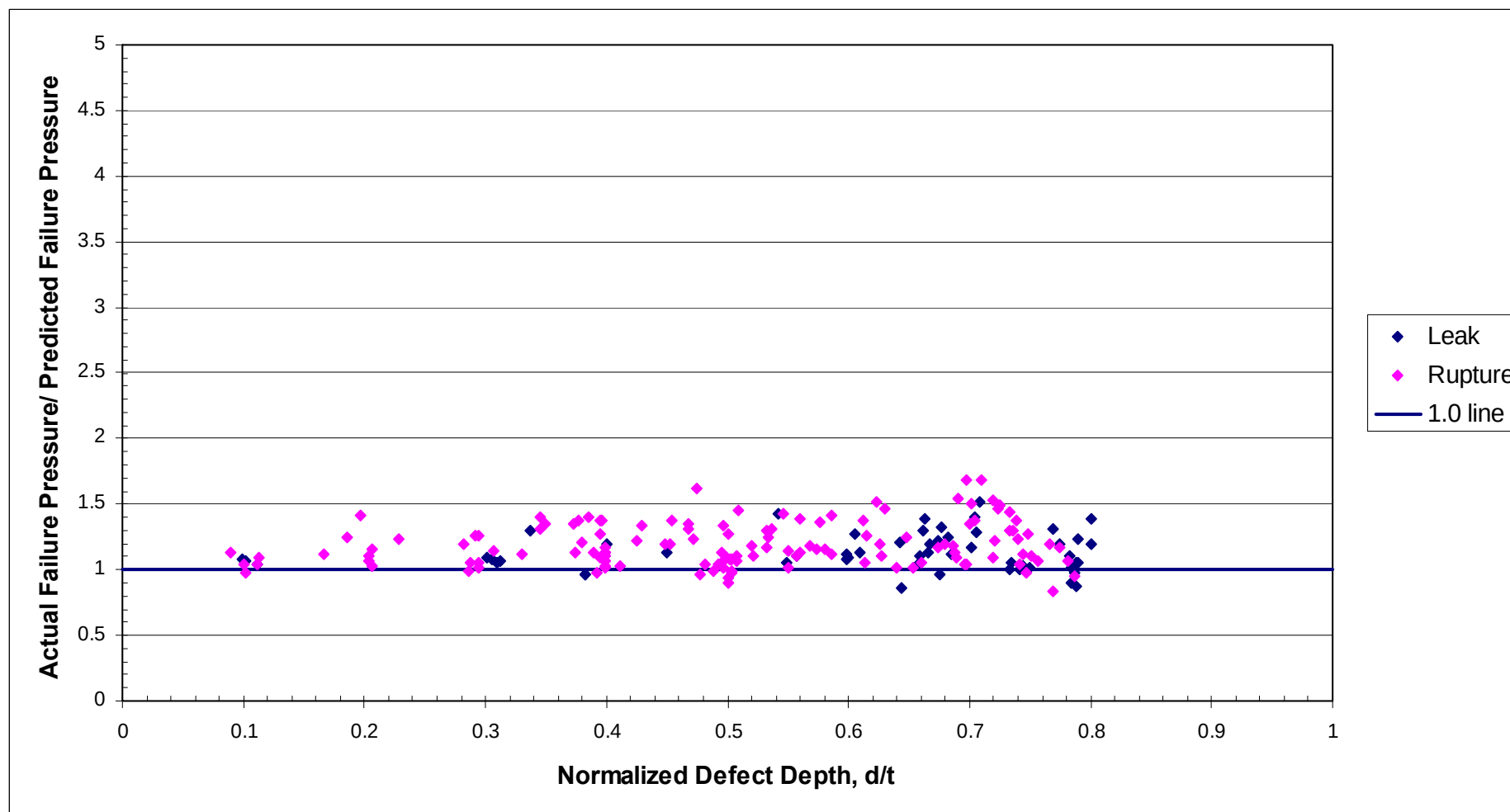
Figure 15 Case 1 Assessments - Comparison of Actual and Predicted Failure Pressures for the Integrated Database Using the RSTRENG Method
