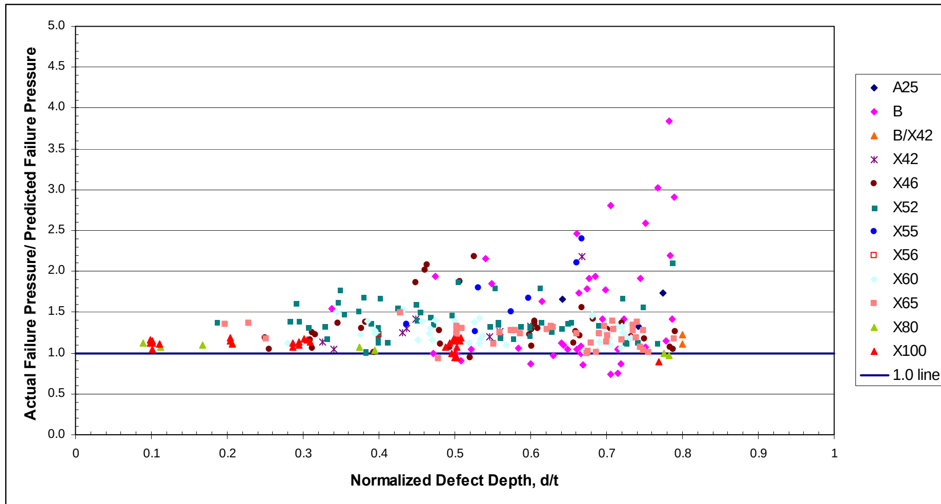
Figure 49 Case 5 Assessments - Comparison of Actual and Predicted Failure Pressures Using the PCORRC Method (Flow Stress Modified to Equal the Mean of the Actual Tensile and Ultimate Tensile Strength)
