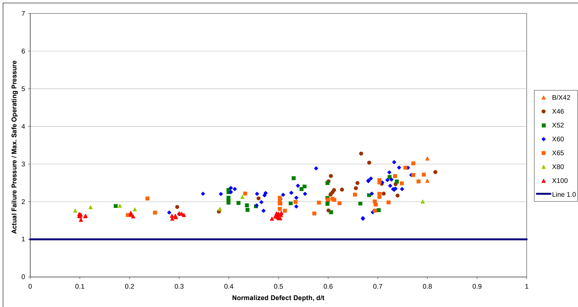
Figure 34 Case 2 Assessments with Factor of Safety 1.39 - Comparison of Actual and Maximum Safe Operating Pressures Using the ASME B31G Method - Machined Defects
