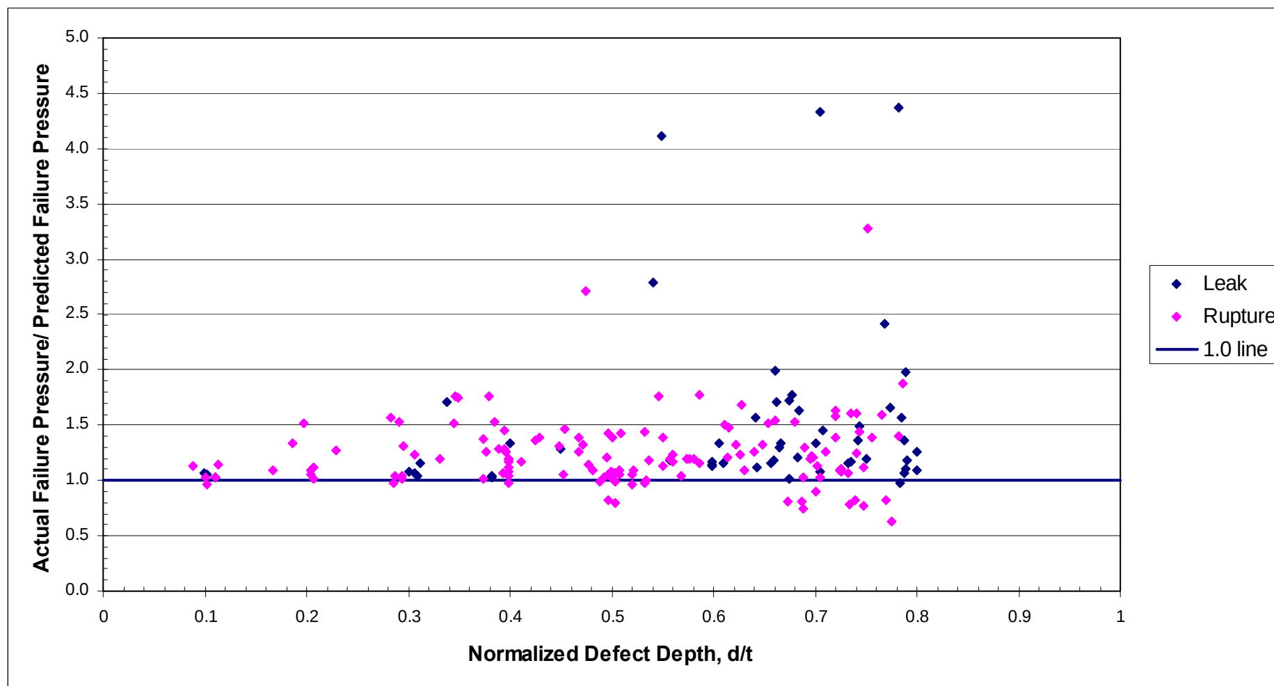
Figure 13 Case 1 Assessments - Comparison of Actual and Predicted Failure Pressures for the Integrated Database Using the ASME B31G Method– Split Between Leaks and Ruptures
