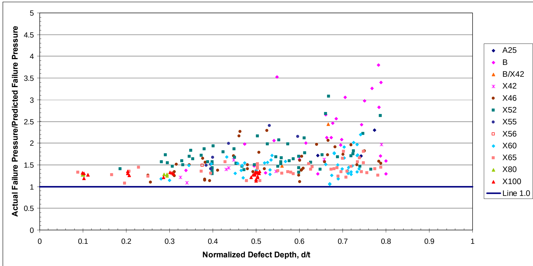
Figure 20 Case 2 Assessments Without a Factor of Safety - Comparison of Actual and Predicted Failure Pressures for the Integrated Database Using the SHELL92 Method
