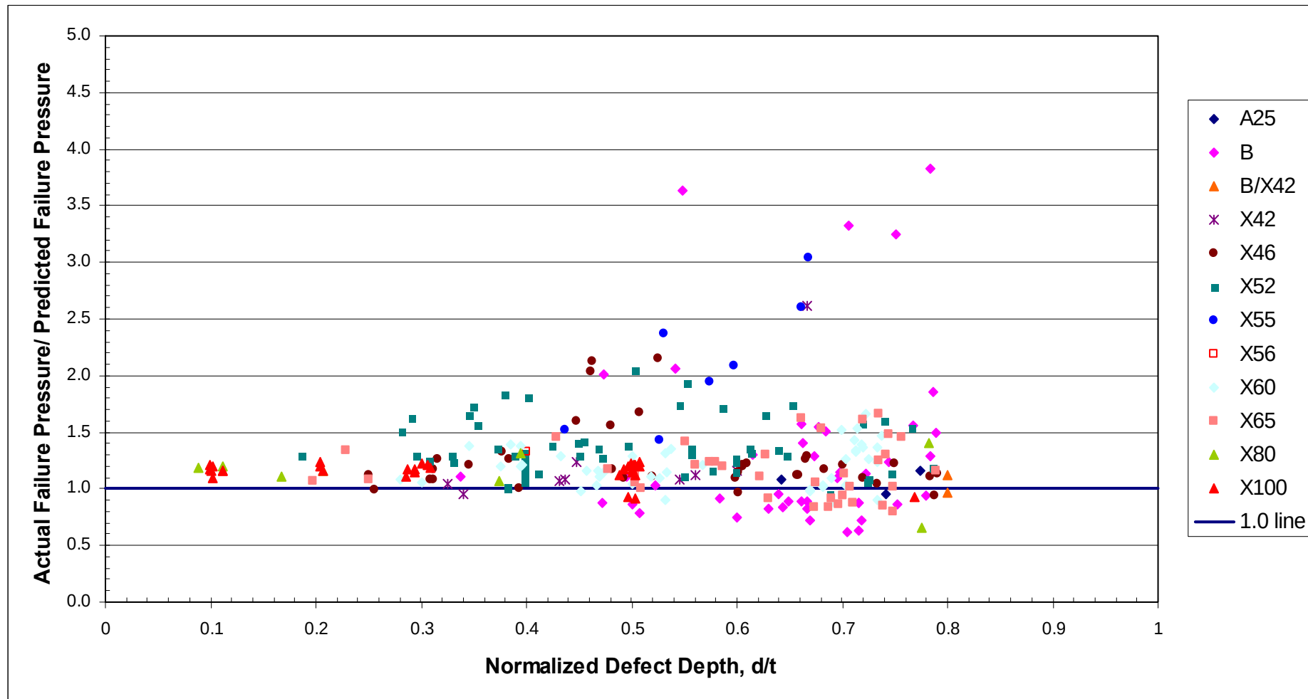
Figure 41 Case 4 Assessments - Comparison of Actual and Predicted Failure Pressures for the Integrated Test Database Using the ASME B31G Method (Flow Stress Modified to Equal the Specified Minimum Tensile Strength)
