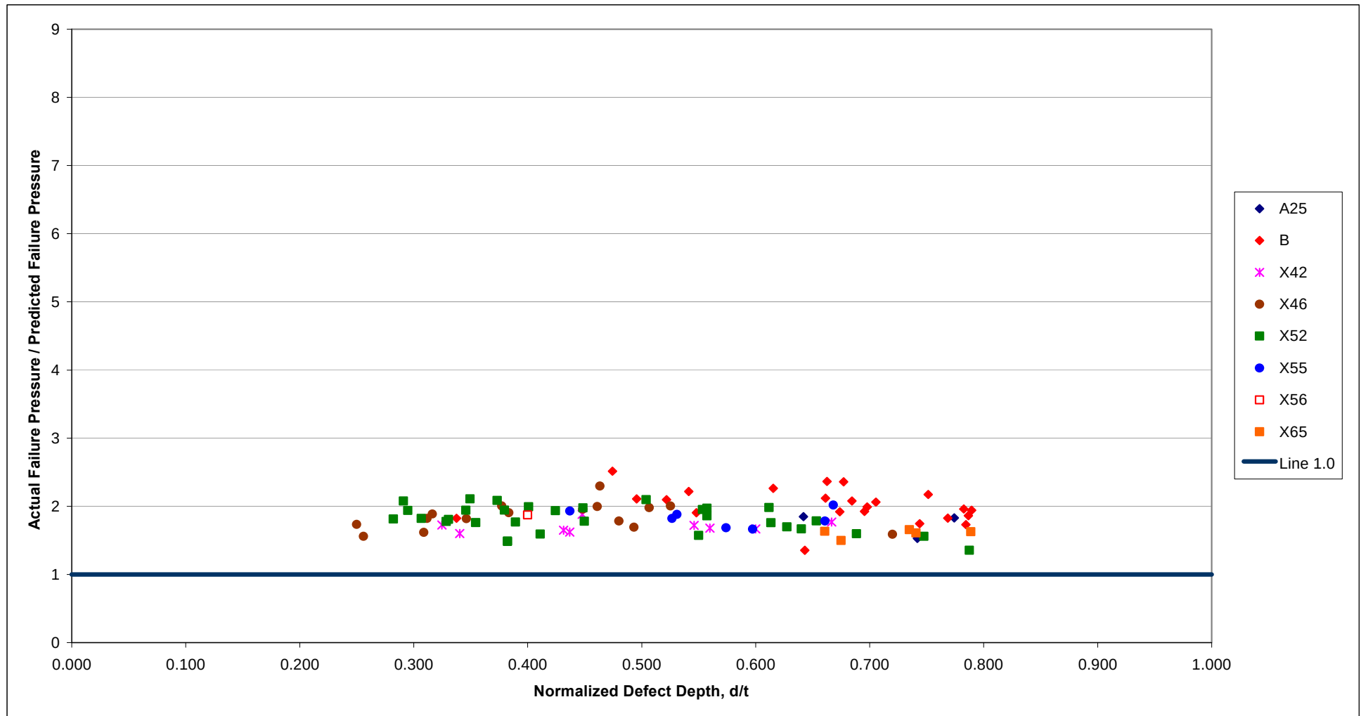
Figure 37 Case 2 Assessments with Factor of Safety 1.39 - Comparison of Actual and Predicted Safe Operating Pressures Using the RSTRENG Method - Real Corrosion Defects
