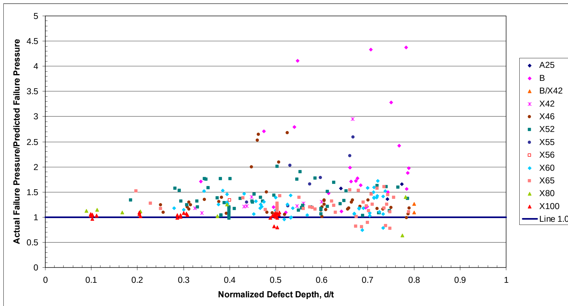
Figure 4 Case 1 Assessments - Comparison of Actual and Predicted Failure Pressures for the Integrated Database Using the ASME B31G Method
