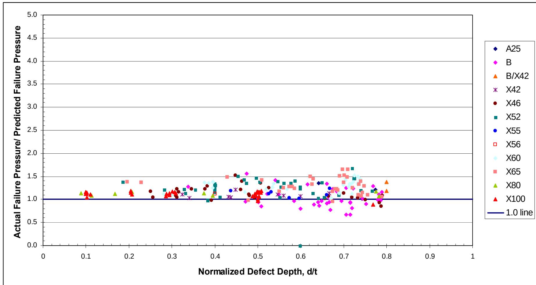
Figure 46 Case 5 Assessments - Comparison of Actual and Predicted Failure Pressures Using the RSTRENG Method (Flow Stress Modified to Equal the Mean of the Actual Tensile and Ultimate Tensile Strength)
