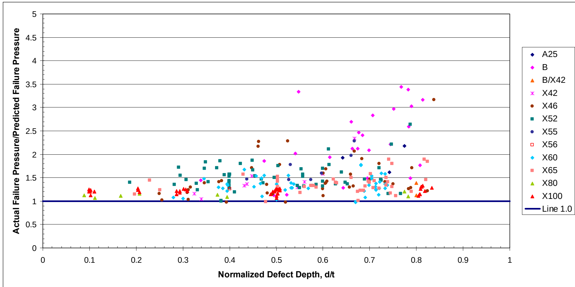
Figure 8 Case 1 Assessments - Comparison of Actual and Predicted Failure Pressure for the Integrated Test Database Using the SHELL92 Method
