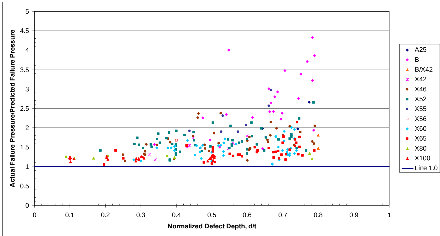
Figure 54 Case 6 Assessments - Comparison of Actual and Predicted Failure Pressures Using the SHELL92 Method (Flow Stress Modified to Equal the Mean of the Specified Minimum Tensile and Ultimate Tensile Strength)
