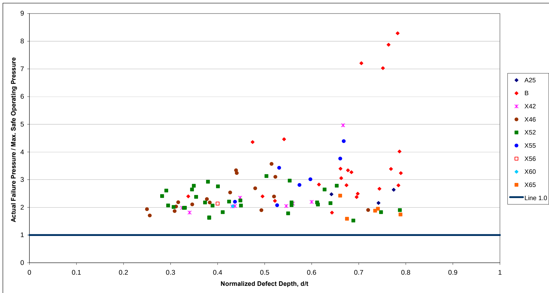
Figure 33 Case 2 Assessments with Factor of Safety 1.39 - Comparison of Actual and Maximum Safe Operating Pressures Using the ASME B31G Method - Real Corrosion Defects
