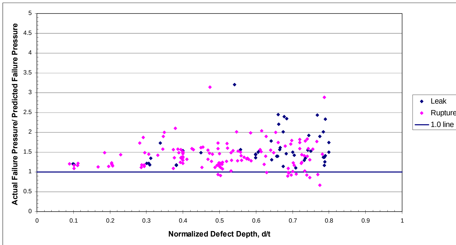
Figure 25 Case 2 Assessments Without a Factor of Safety - Comparison of Actual and Predicted Failure Pressures for the Integrated Database Using the ASME B31G Method – Split Between Leaks and Ruptures
