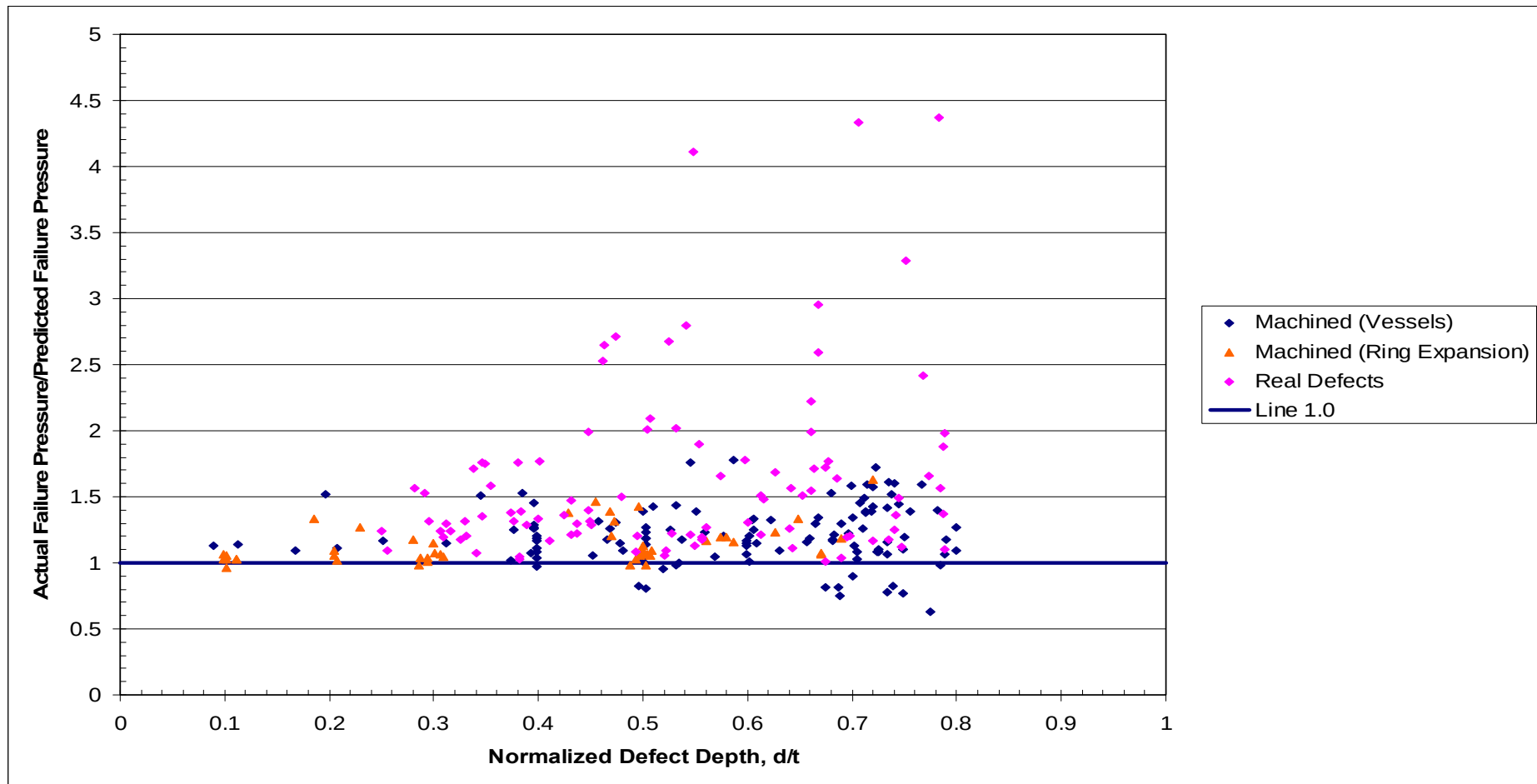
Figure 10 Case 1 Assessments - Comparison of Actual and Predicted Failure Pressures for the Integrated Database Using the ASME B31G Method – Split Between Machined and Real Corrosion Defects
