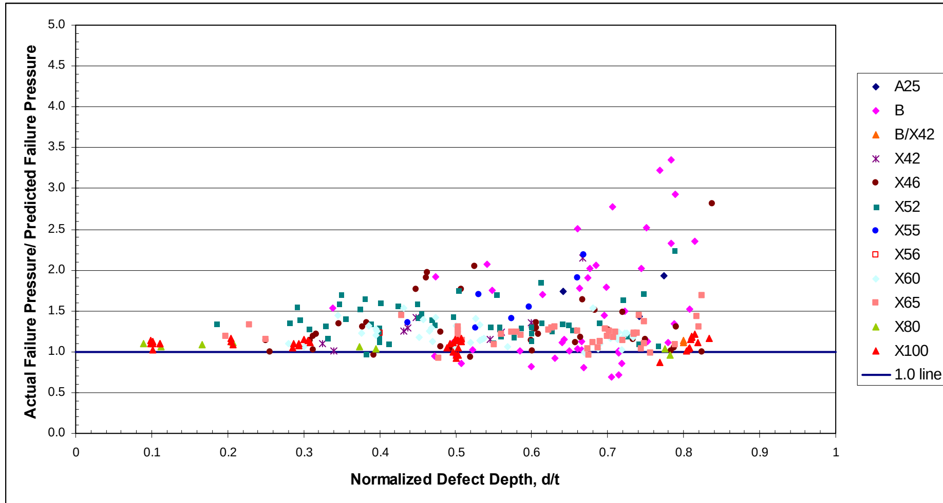
Figure 47 Case 5 Assessments - Comparison of Actual and Predicted Failure Pressures Using the LPC-1 Method (Flow Stress Modified to Equal the Mean of the Actual Tensile and Ultimate Tensile Strength)
