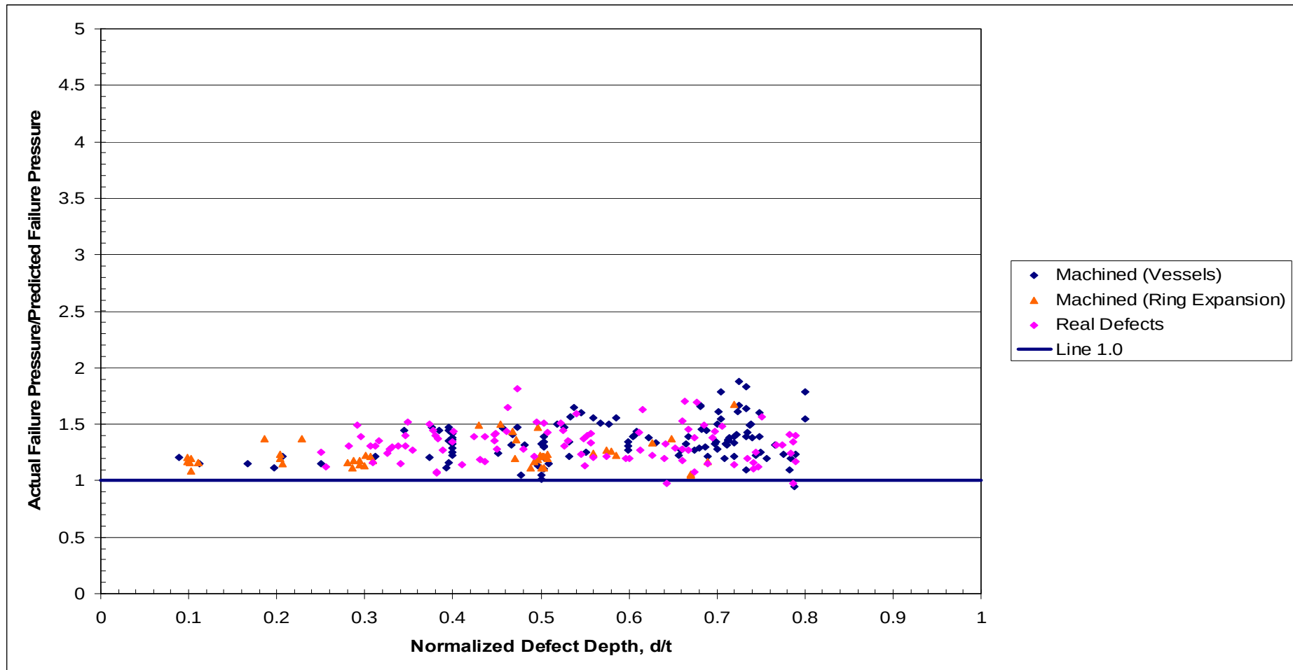
Figure 24 Case 2 Assessments Without a Factor of Safety - Comparison of Actual and Predicted Failure Pressure for the Integrated Database Using the RSTRENG Method – Split Between Machined and Real Corrosion Defects
