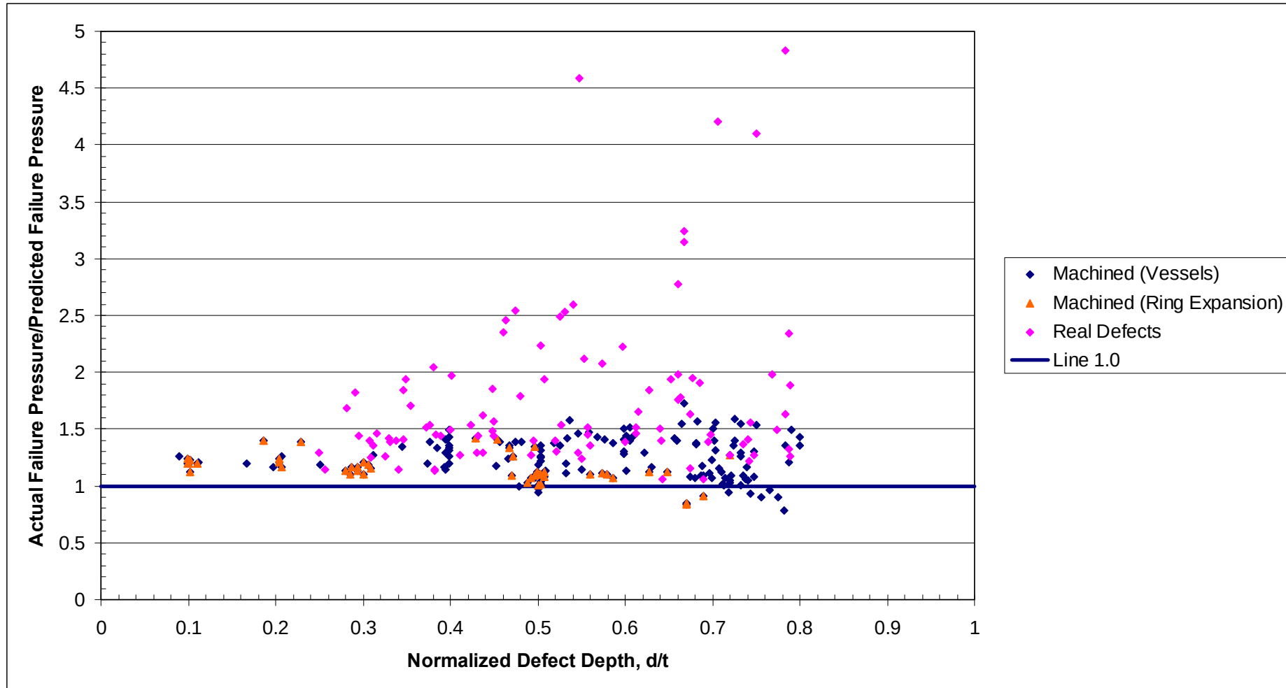
Figure 57 Case 6 Assessments - Comparison of Actual and Predicted Failure Pressure Using the Modified ASME B31G Method (Flow Stress Modified to Equal the Mean of the Specified Minimum Tensile and Ultimate Tensile Strength) – Split Between Machined and Real Corrosion Defects
