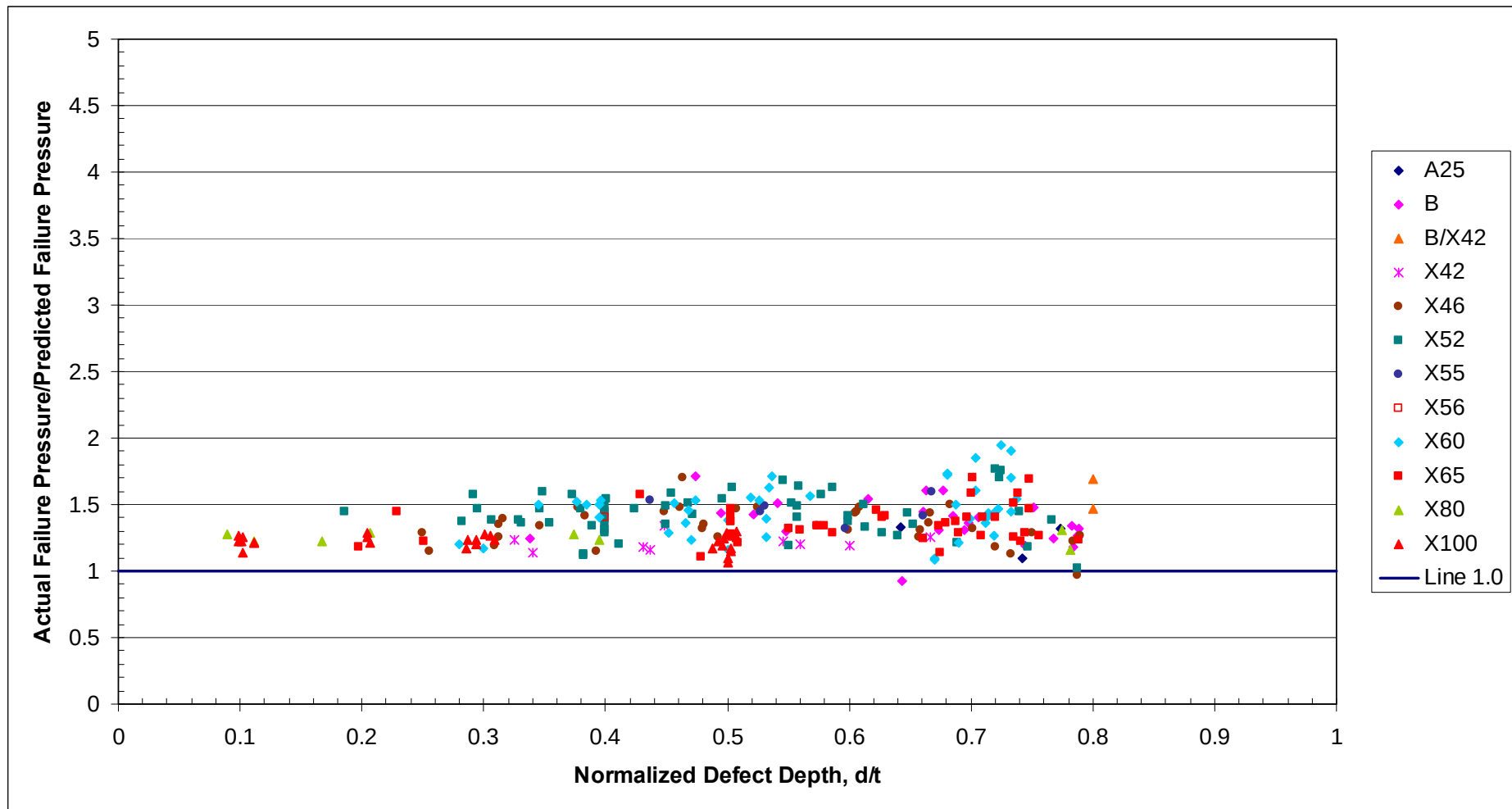
Figure 52 Case 6 Assessments - Comparison of Actual and Predicted Failure Pressures Using the RSTRENG Method (Flow Stress Modified to Equal the Mean of the Specified Minimum Tensile and Ultimate Tensile Strength)
