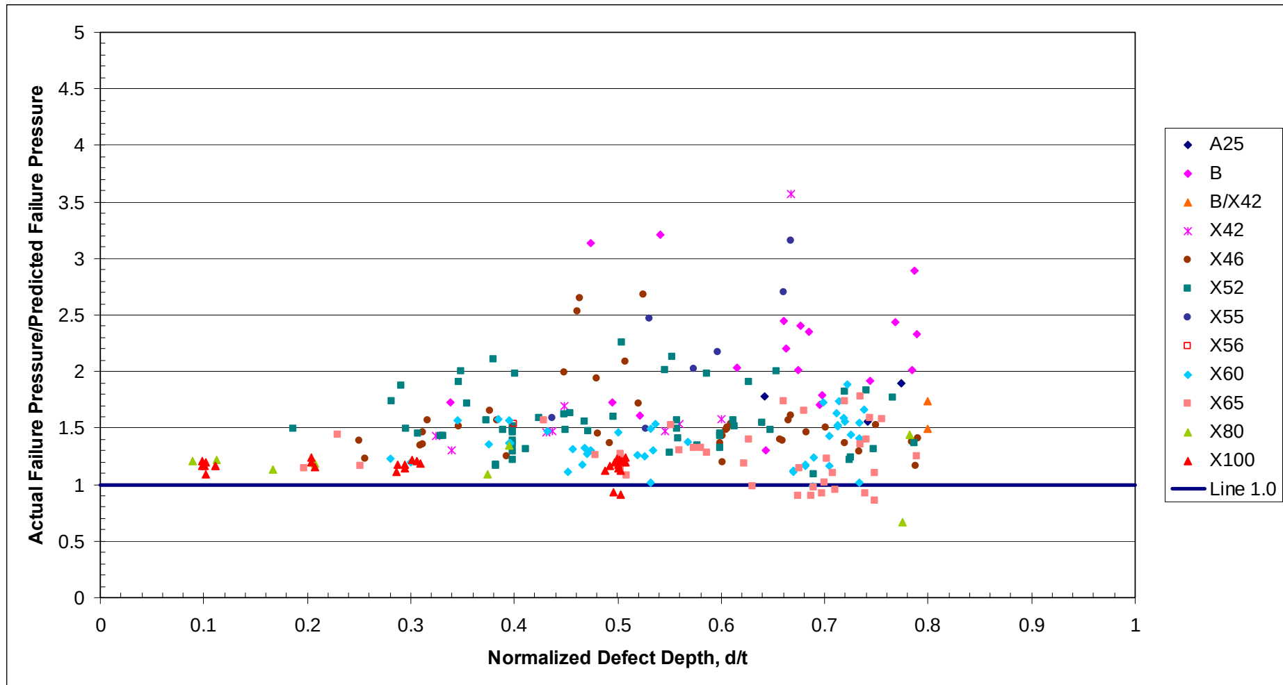
Figure 16 Case 2 Assessments Without a Factor of Safety - Comparison of Actual and Predicted Failure Pressures for the Integrated Database Using the ASME B31G Method
