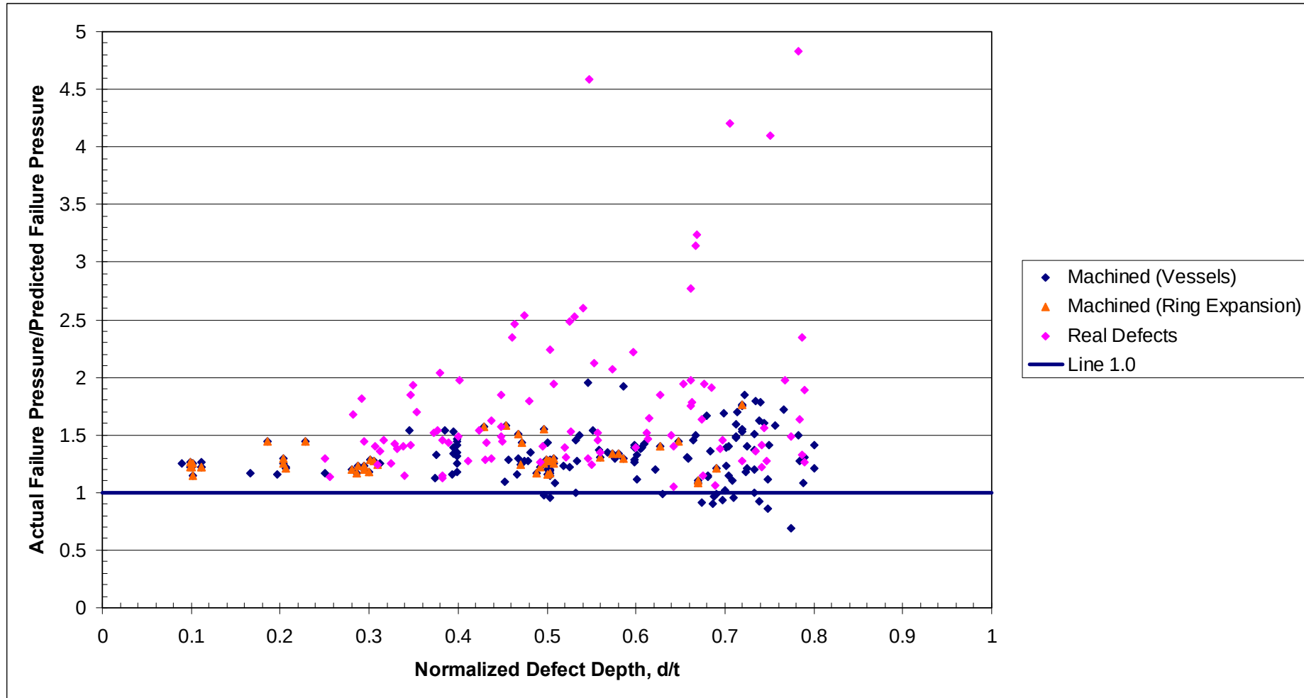
Figure 56 Case 6 Assessments - Comparison of Actual and Predicted Failure Pressure Using the ASME B31G Method (Flow Stress Modified to Equal the Mean of the Specified Minimum Tensile and Ultimate Tensile Strength) – Split Between Machined and Real Corrosion Defects
