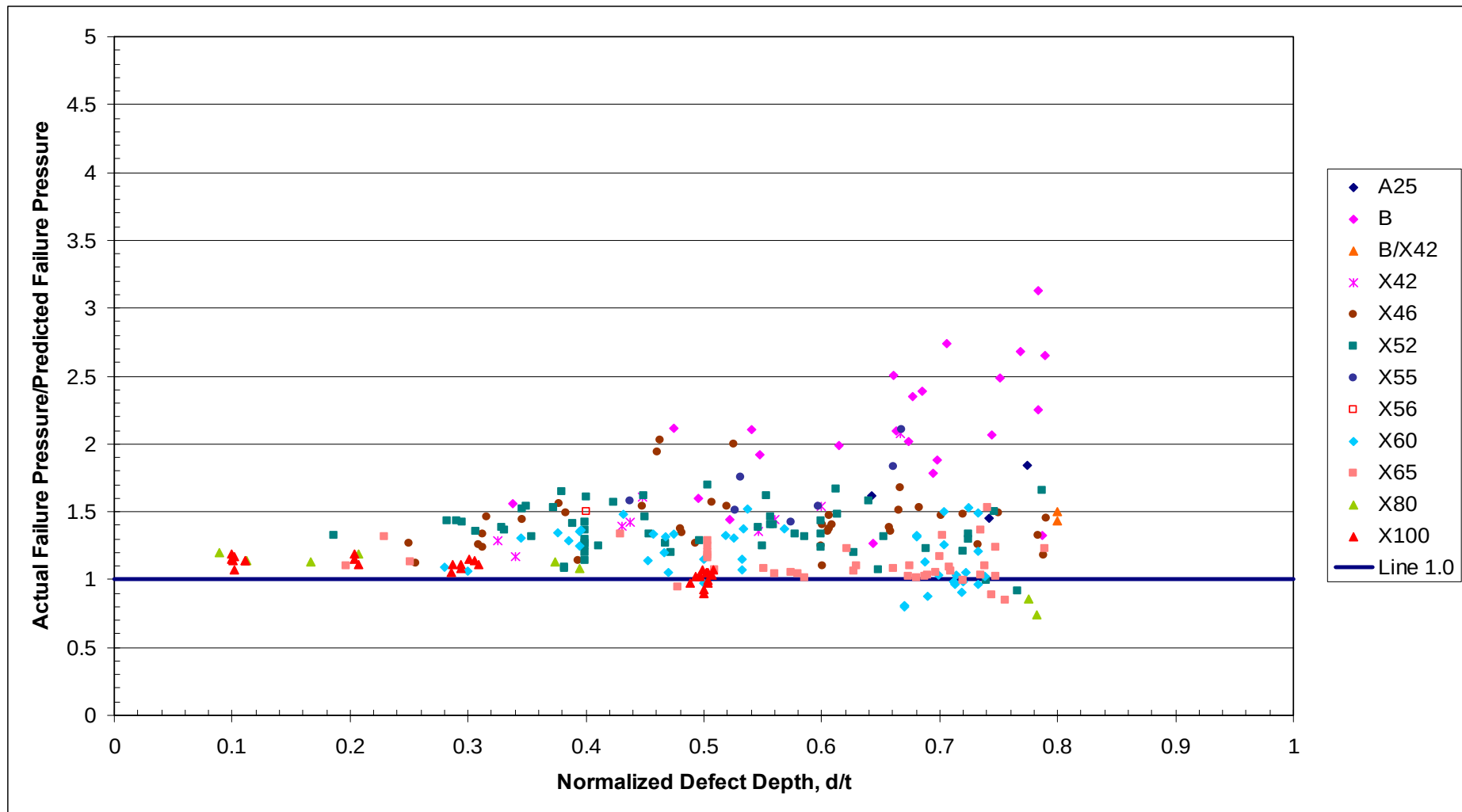
Figure 17 Case 2 Assessments Without a Factor of Safety - Comparison of Actual and Predicted Failure Pressures for the Integrated Database Using the Modified ASME B31G Method (Including Ring Expansion Tests)
