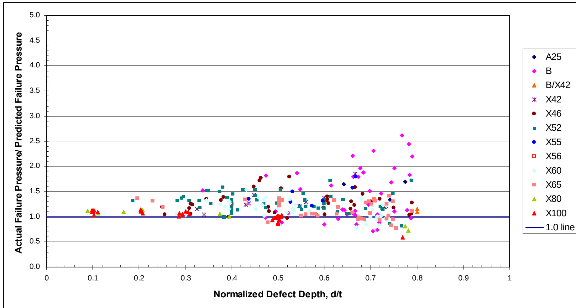
Figure 45 Case 5 Assessments - Comparison of Actual and Predicted Failure Pressures for the Integrated Test Database Using the Modified ASME B31G Method (Flow Stress Modified to Equal the Mean of the Actual Tensile and Ultimate Tensile Strength, including Ring Expansion Tests)
