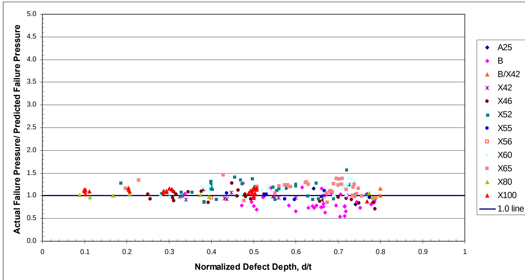
Figure 40 Case 3 Assessments - Comparison of Actual and Predicted Failure Pressures for the Integrated Test Database Using the RSTRENG Method (Flow Stress Modified to Equal the Actual Tensile Strength)
