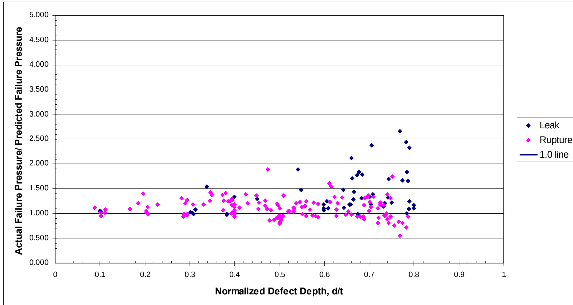
Figure 14 Case 1 Assessments - Comparison of Actual and Predicted Failure Pressures for the Integrated Database Using the Modified ASME B31G Method (Including Ring Expansion Tests) – Split Between Leaks and Ruptures
