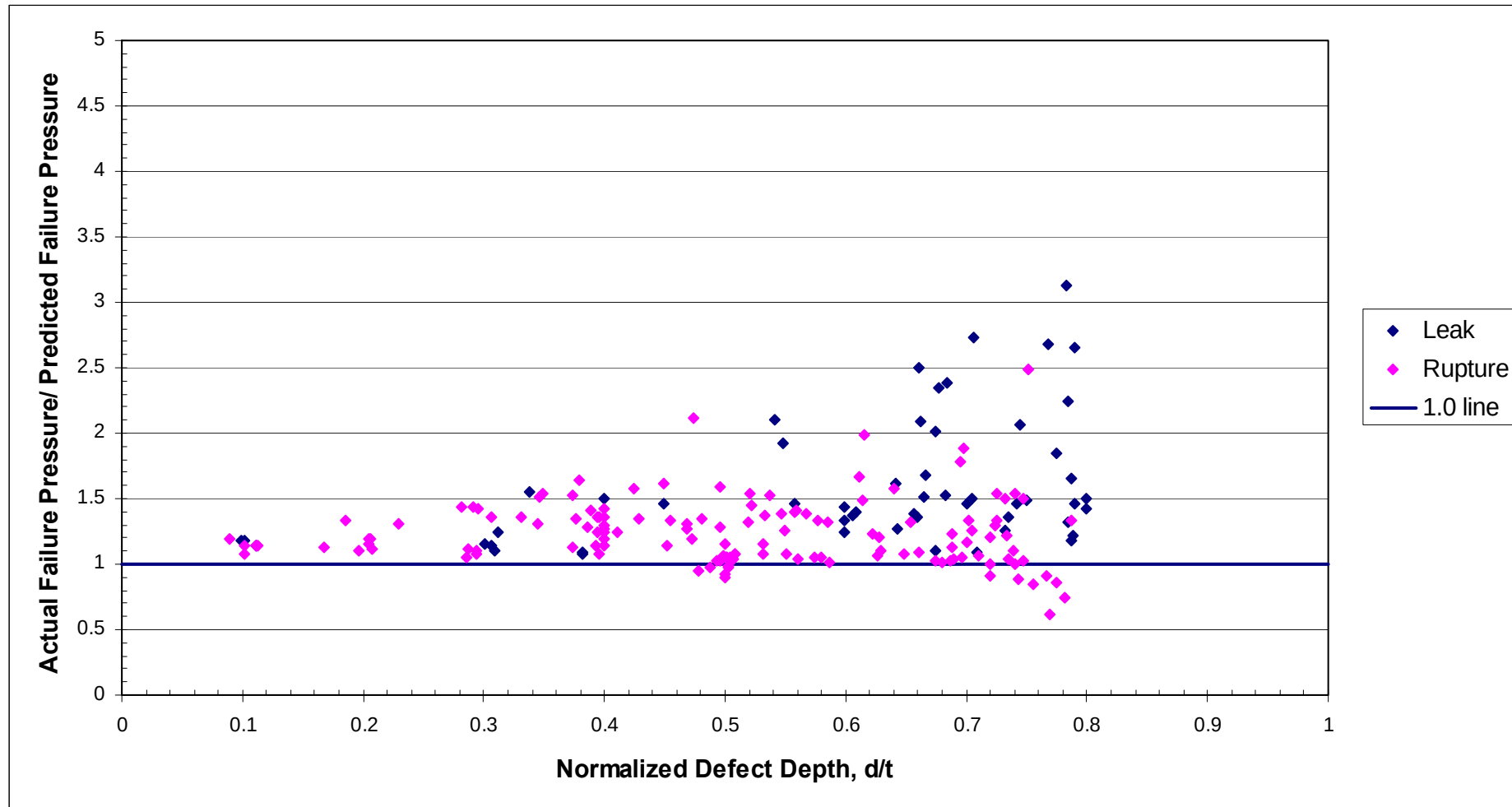
Figure 26 Case 2 Assessments Without a Factor of Safety - Comparison of Actual and Predicted Failure Pressures for the Integrated Database Using the Modified ASME B31G Method (Including Ring Expansion Tests) – Split Between Leaks and Ruptures
