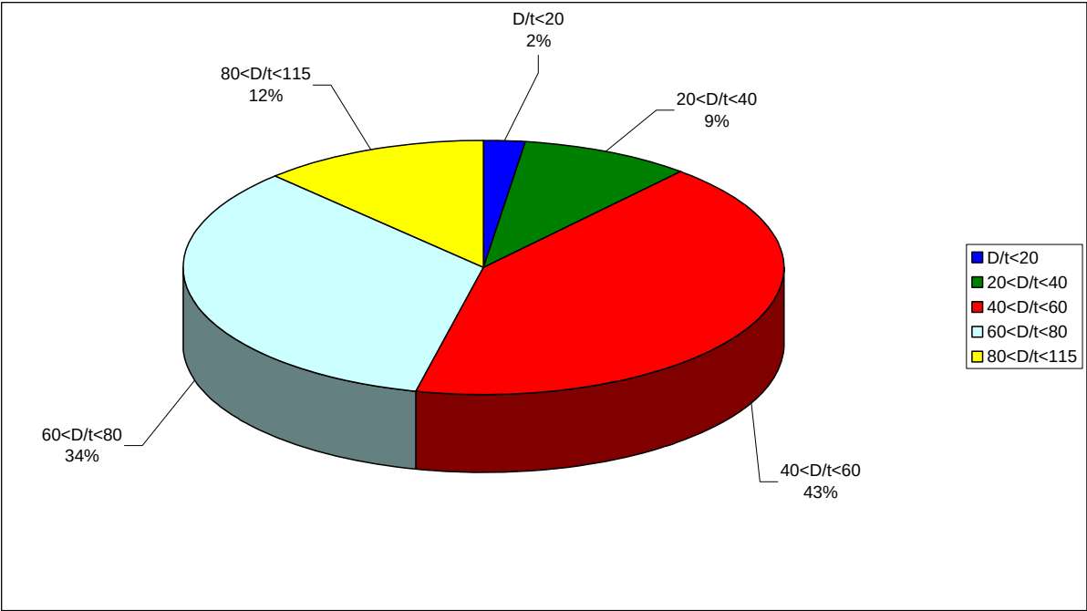
Figure 2 Pipe Diameter to Thickness (D/t) Ratios Covered in the Integrated Test Database
