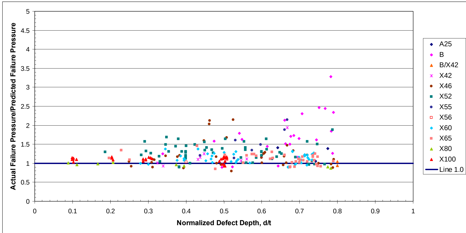
Figure 9 Case 1 Assessments - Comparison of Actual and Predicted Failure Pressure for the Integrated Test Database Using the PCORRC Method
