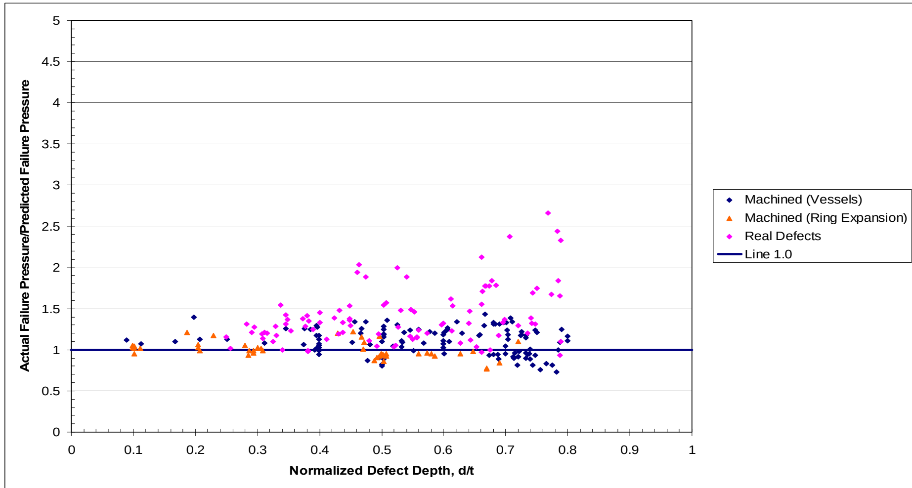
Figure 11 Case 1 Assessments - Comparison of Actual and Predicted Failure Pressure for the Integrated Test Database Using the Modified ASME B31G Method (Including Ring Expansion Tests) – Split Between Machined and Real Corrosion Defects
