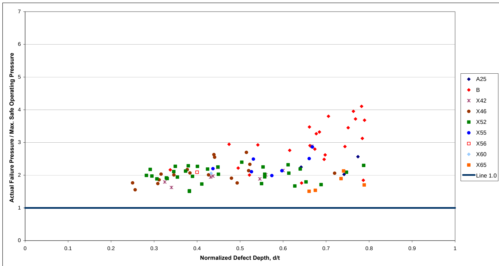
Figure 35 Case 2 Assessments with Factor of Safety 1.39 - Comparison of Actual and Maximum Safe Operating Pressures Using the Modified ASME B31G Method - Real Corrosion Defects
