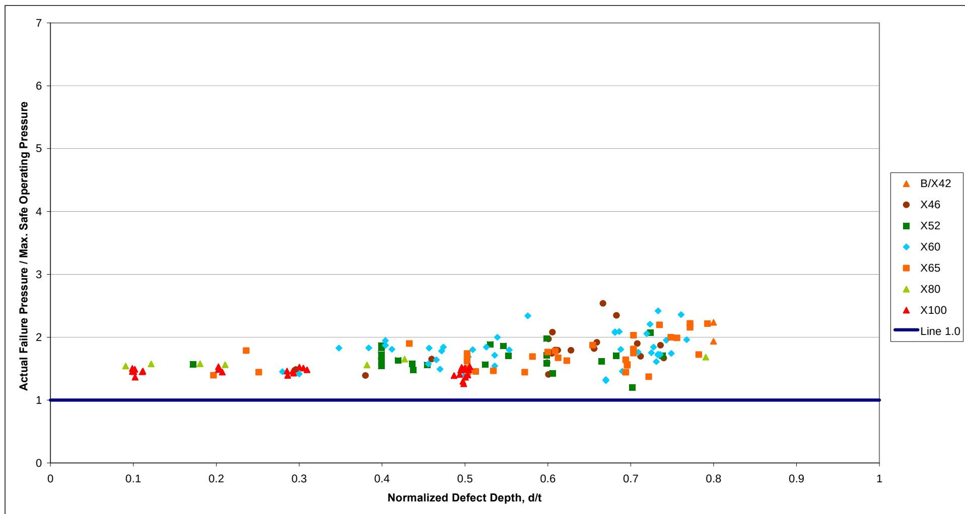
Figure 31 Case 2 Assessments with Factor of Safety 1.25 - Comparison of Actual and Predicted Safe Operating Pressures Using the Modified ASME B31G Method - Machined Defects
