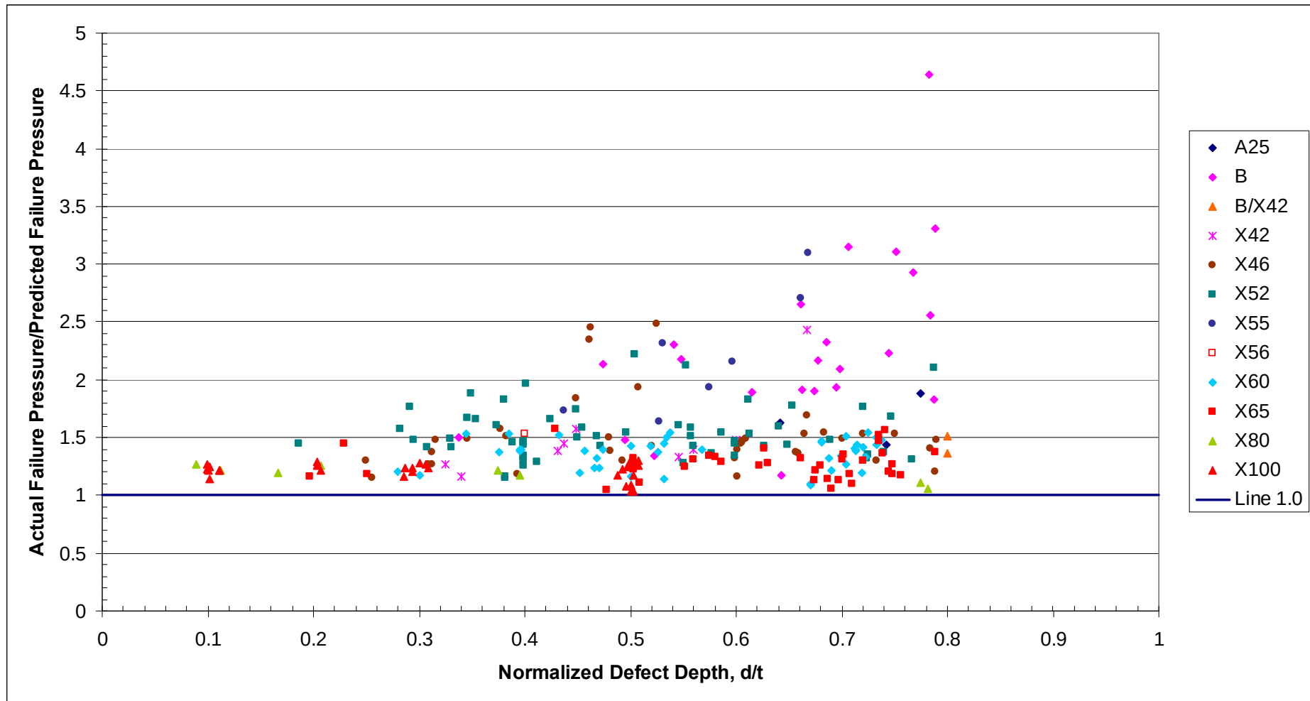
Figure 55 Case 6 Assessments - Comparison of Actual and Predicted Failure Pressures Using the PCORRC Method (Flow Stress Modified to Equal the Mean of the Specified Minimum Tensile and Ultimate Tensile Strength)
