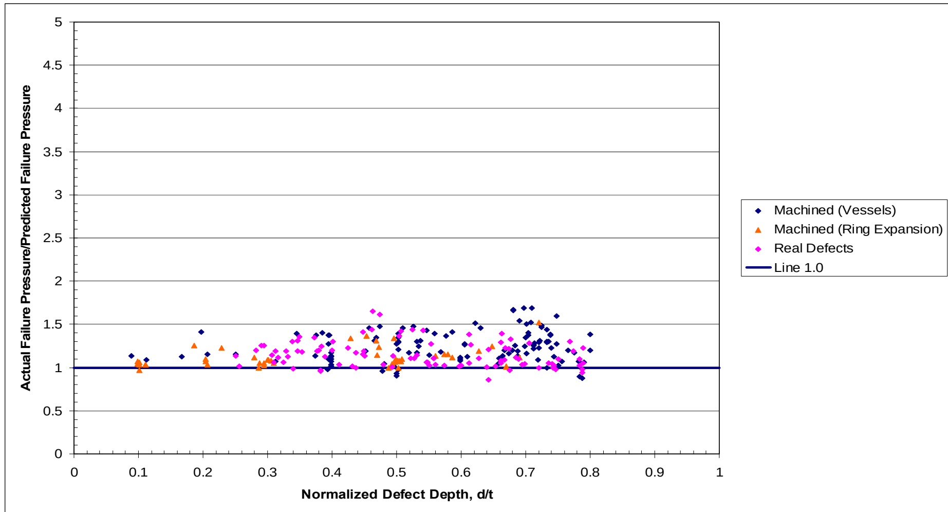
Figure 12 Case 1 Assessments - Comparison of Actual and Predicted Failure Pressure for the Integrated Test Database Using the RSTRENG Method – Split Between Machined and Real Corrosion Defects
