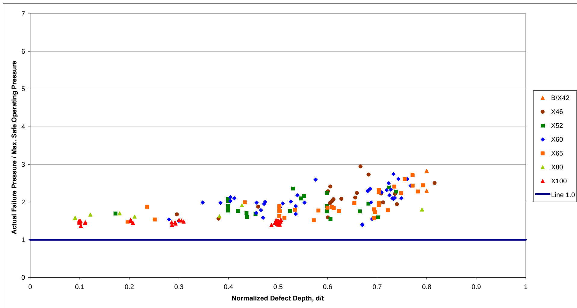
Figure 29 Case 2 Assessments with Factor of Safety 1.25 - Comparison of Actual and Maximum Safe Operating Pressures Using the ASME B31G Method - Machined Defects
