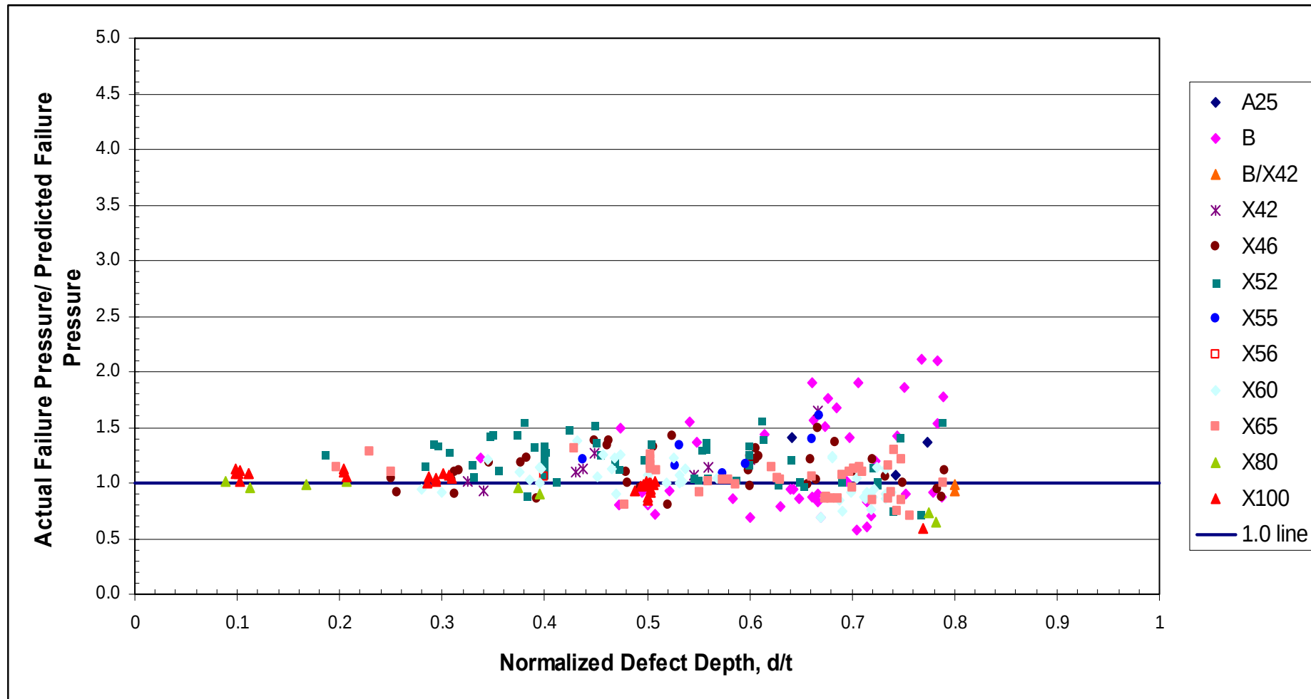
Figure 39 Case 3 Assessments - Comparison of Actual and Predicted Failure Pressures for the Integrated Test Database Using the Modified ASME B31G Method (Flow Stress Modified to Equal the Actual Tensile Strength, including Ring Expansion Tests)
