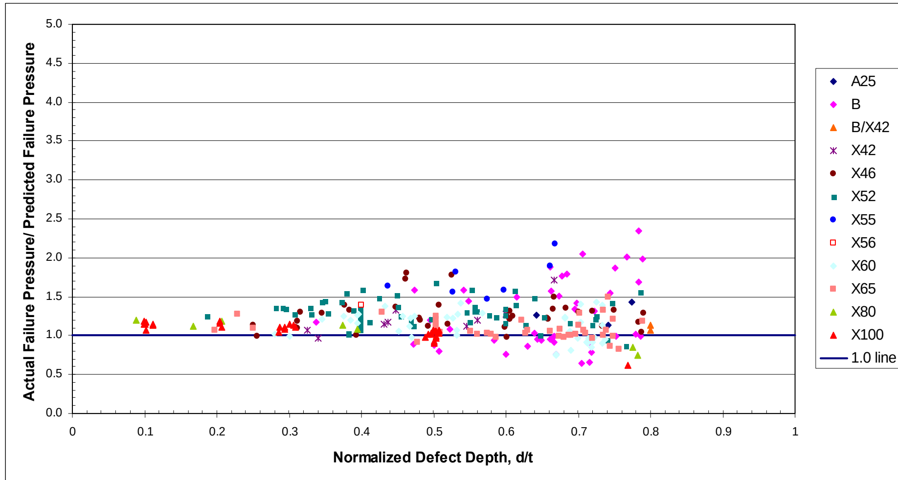
Figure 42 Case 4 Assessments - Comparison of Actual and Predicted Failure Pressures for the Integrated Test Database Using the Modified ASME B31G Method (Flow Stress Modified to Equal the Specified Minimum Tensile Strength, including Ring Expansion Tests)
