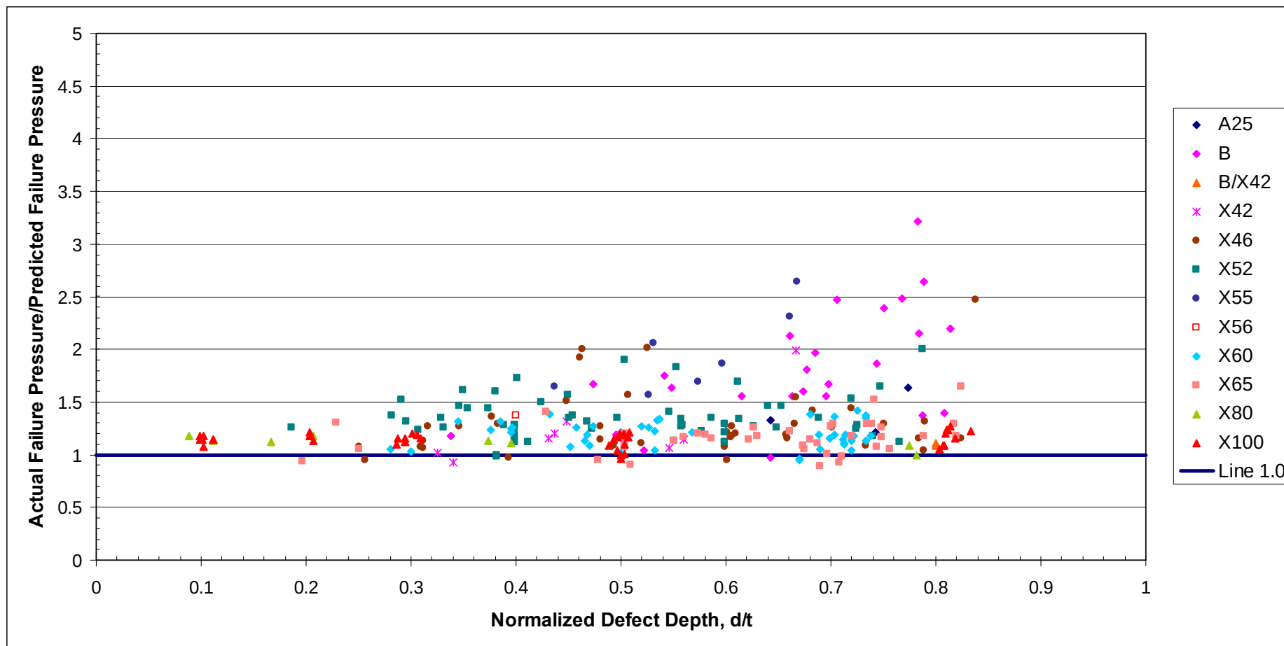
Figure 19 Case 2 Assessments Without a Factor of Safety - Comparison of Actual and Predicted Failure Pressures for the Integrated Database Using the LPC-1 Method
