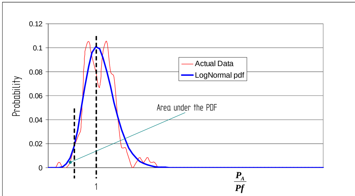
Figure 59 Probability Density Function of (P_A/P_f)
