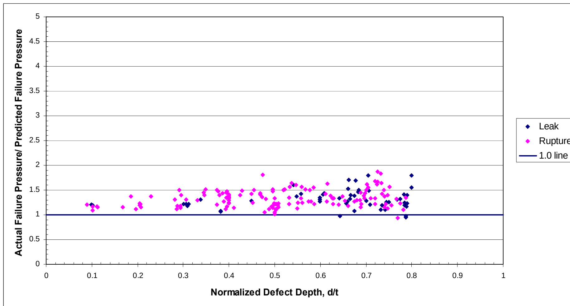
Figure 27 Case 2 Assessments Without a Factor of Safety - Comparison of Actual and Predicted Failure Pressures for the Integrated Database Using the RSTRENG Method – Split Between Leaks and Ruptures
