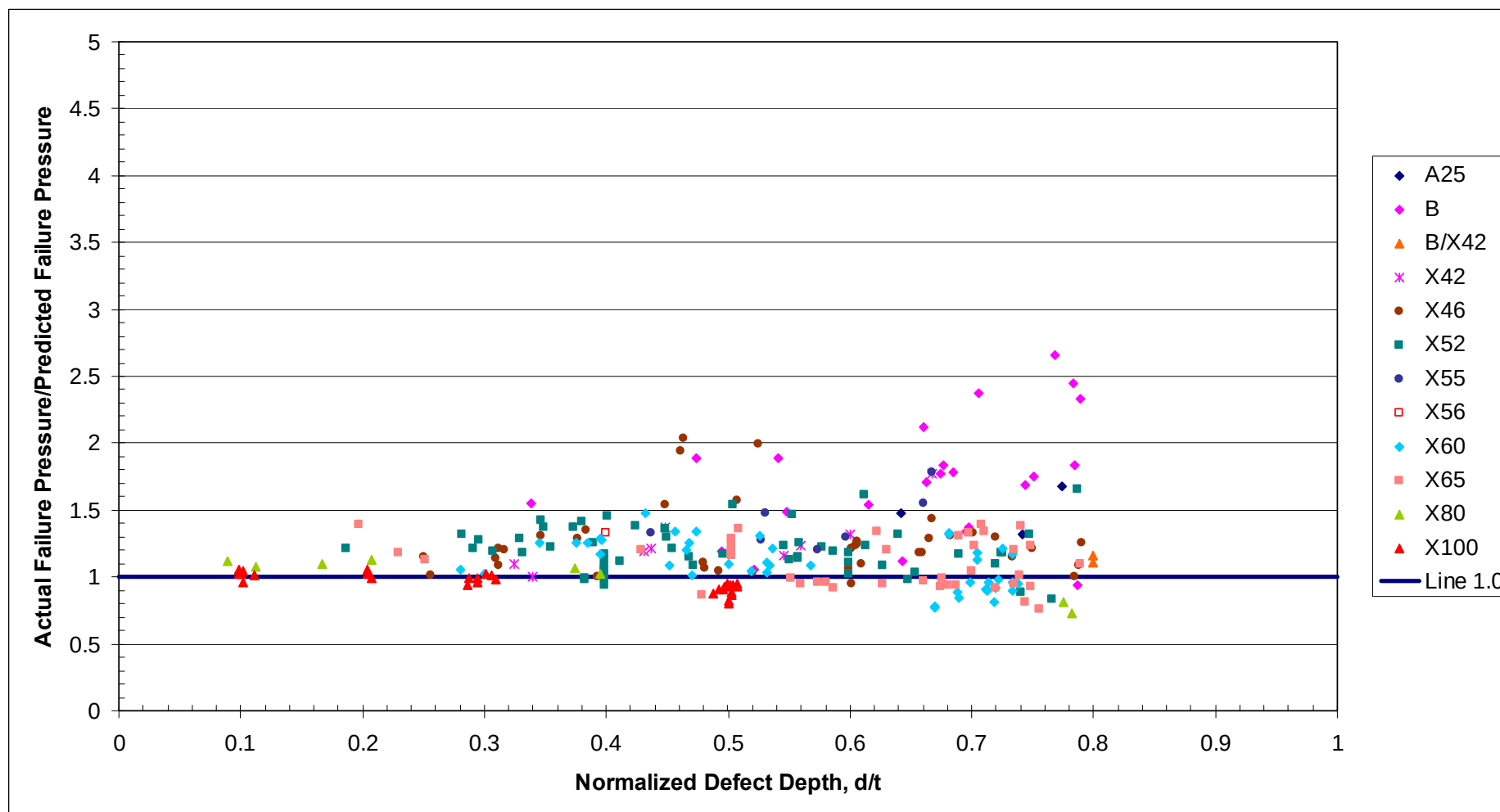
Figure 5 Case 1 Assessments - Comparison of Actual and Predicted Failure Pressure for the Integrated Test Database Using the Modified ASME B31G Method (Including Ring Expansion Tests)
