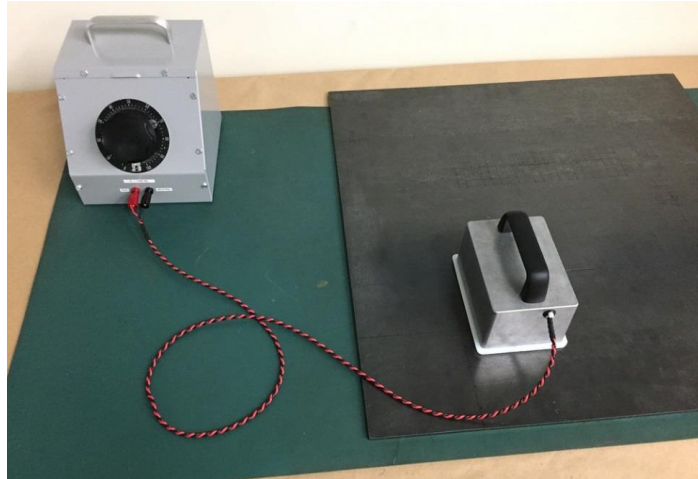
FIGURE 7: APPARATUS TO DE-MAGNETIZE STEEL PLATE AND PIPE SAMPLES
