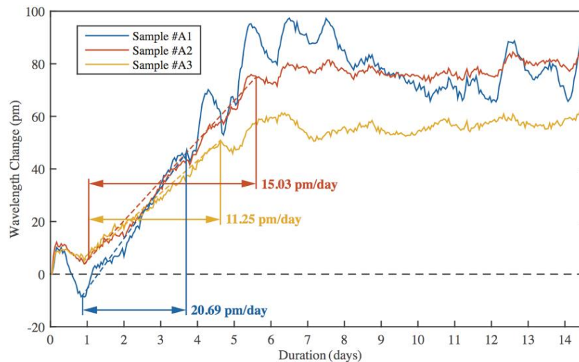
Figure 61. Corrosion rate of three coated samples shown on graph.
