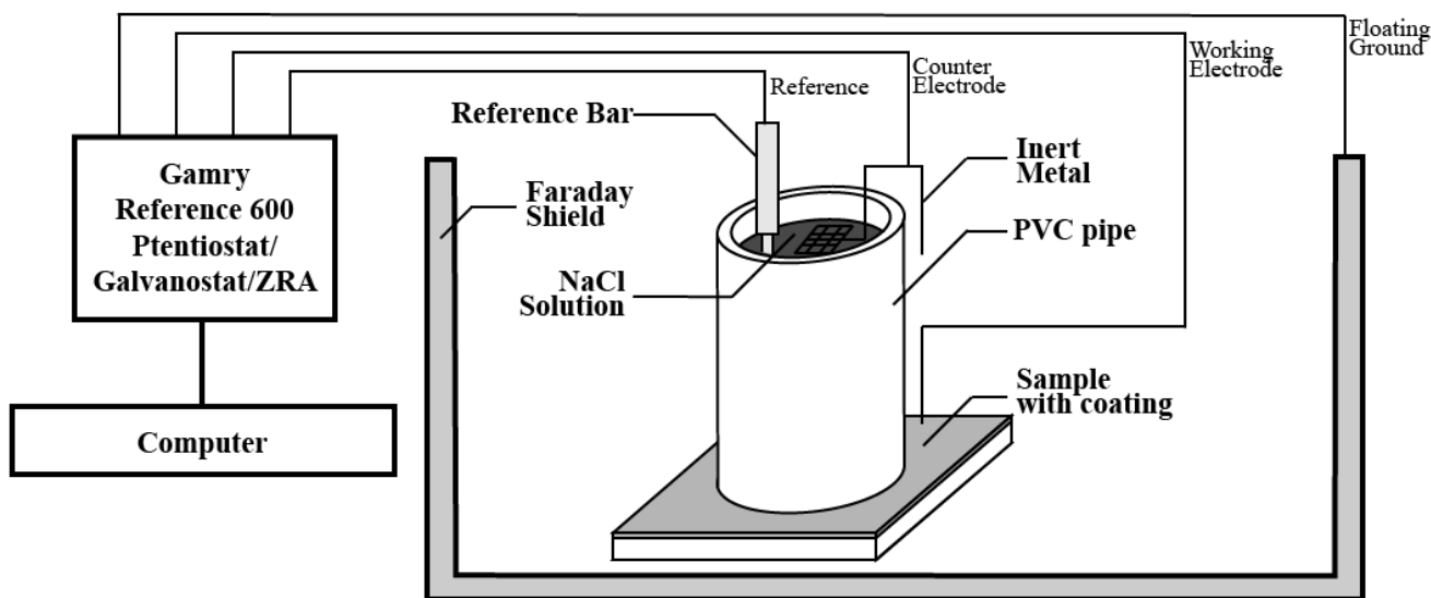
Figure 32. Schematic of the accelerated electrochemical corrosion test setup.
