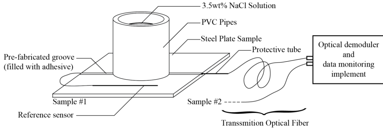
Figure 49. Schematic of an accelerated corrosion test set-up.
