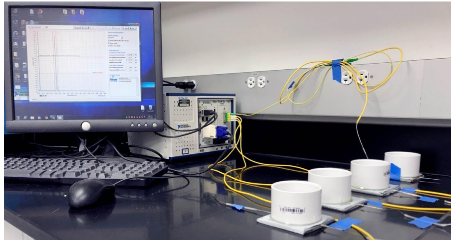
Figure 58. Integrated system in accelerated corrosion test setup.
