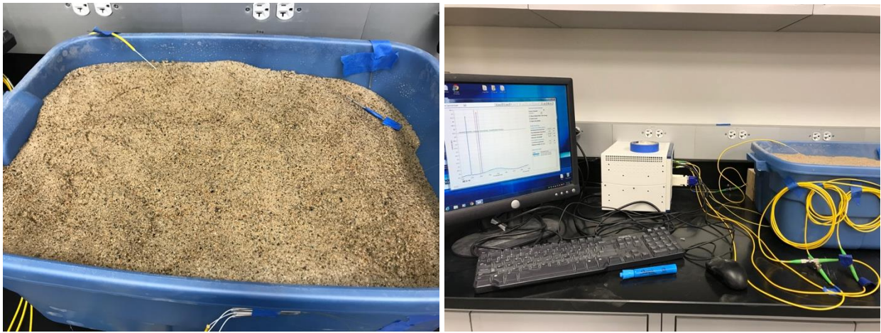
Figure 83. Experiment setup for the steel pipe sample coated with soft coating.
