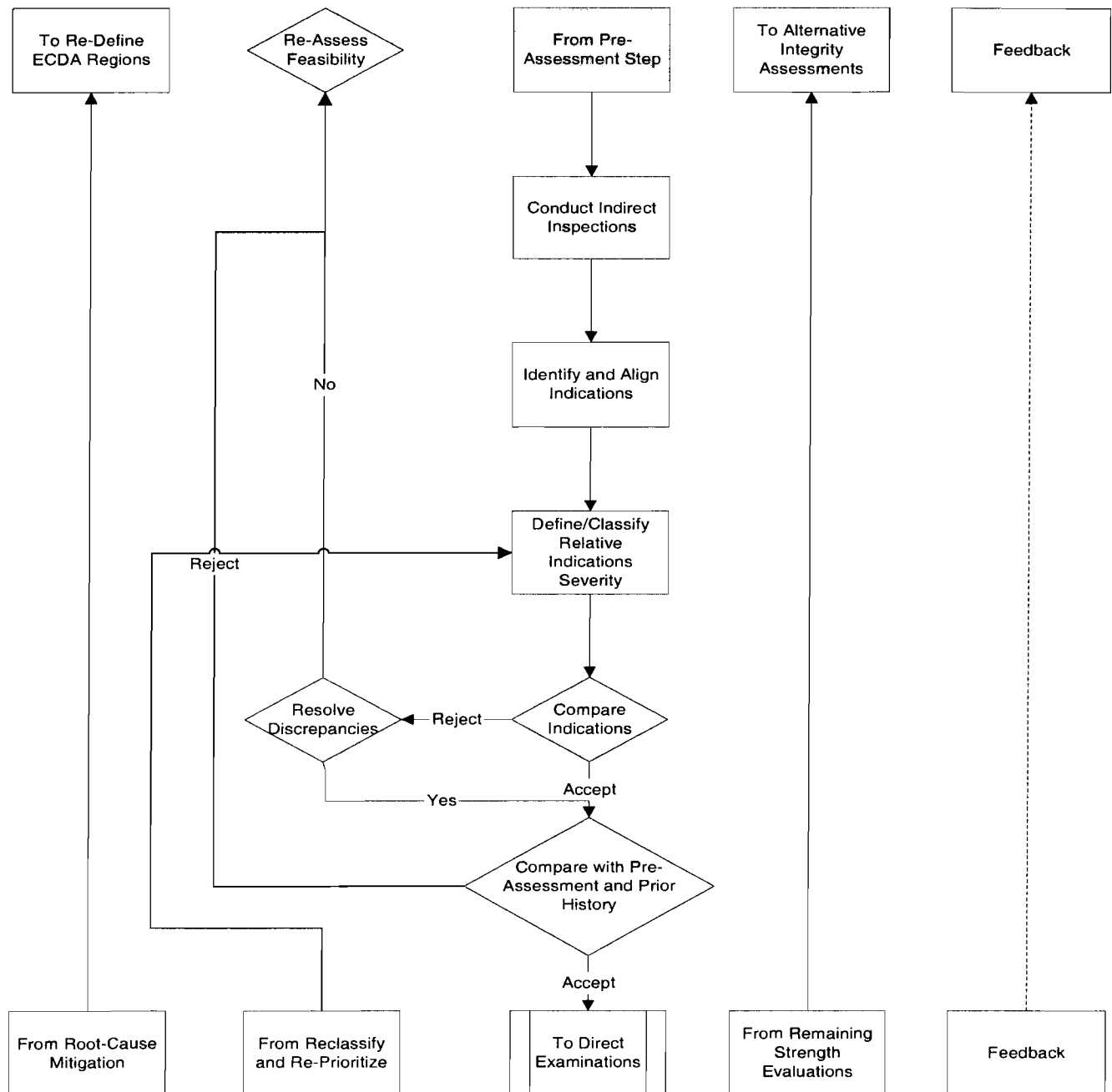
Figure A3.2: Indirect Inspection Flow Chart (continuation of Fig. A3.1: Pre-Assessment Flow Chart)
