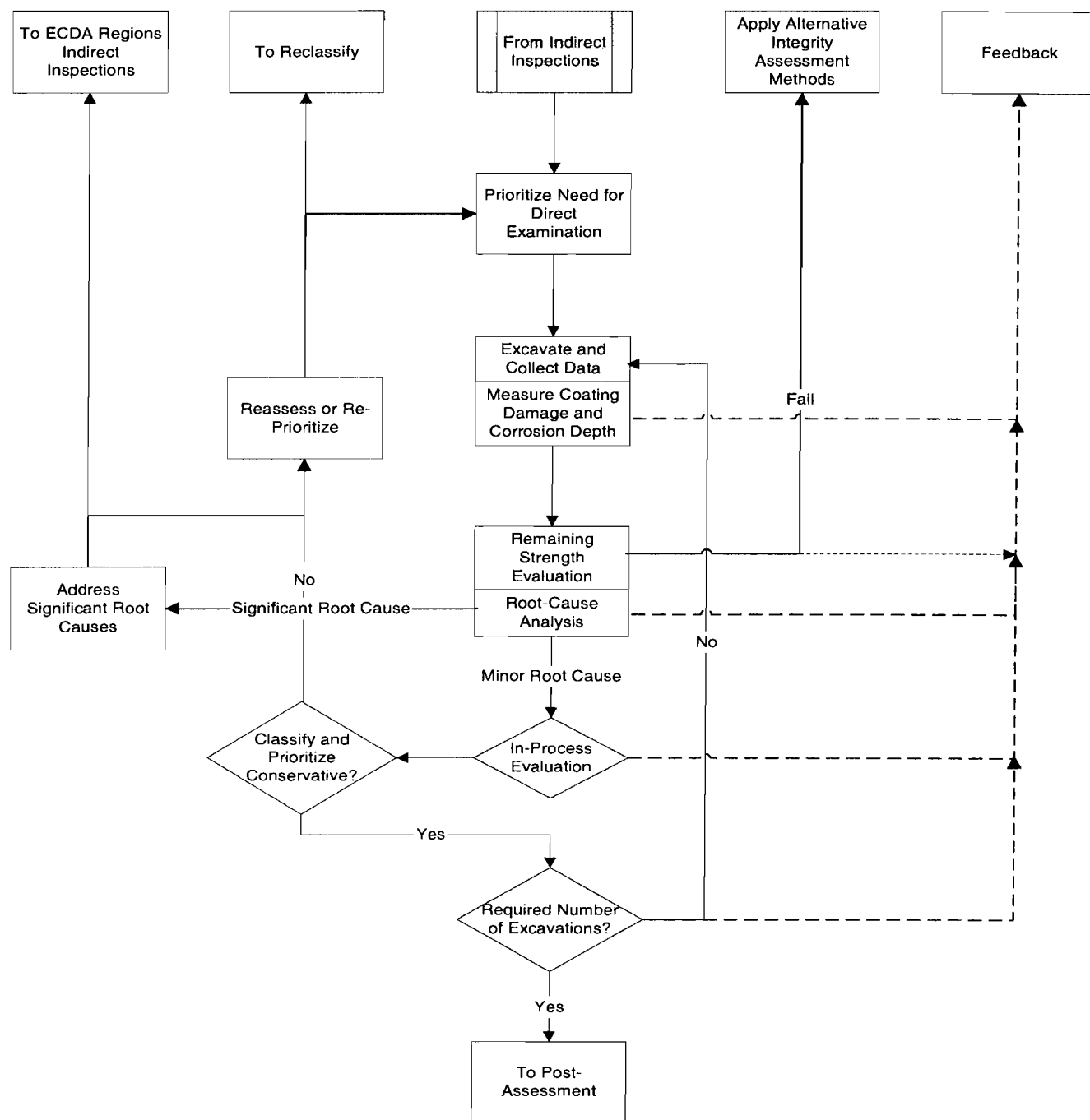
Figure A3.3: Direct Examination Flow Chart (continuation of Figure A3.2: Indirect Inspection Flow Chart)
