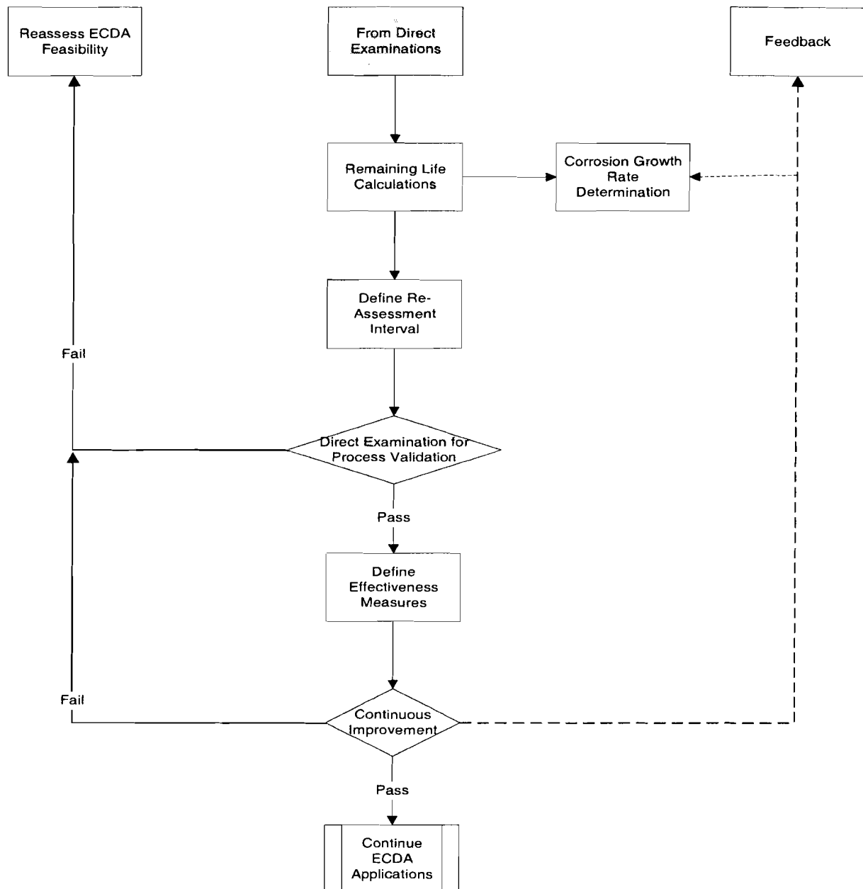
Figure A3.4: Post-Assessment Flow Chart (continued from Figure A3.3: Direct Examination Flow Chart)
