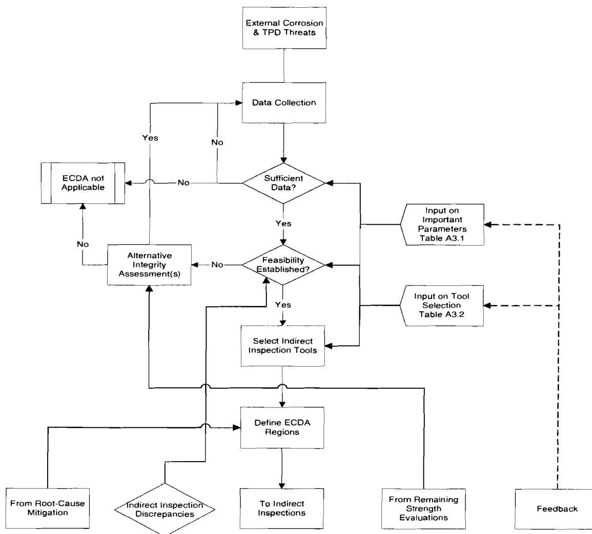
Figure A3.1: Pre-Assessment Flow Chart
